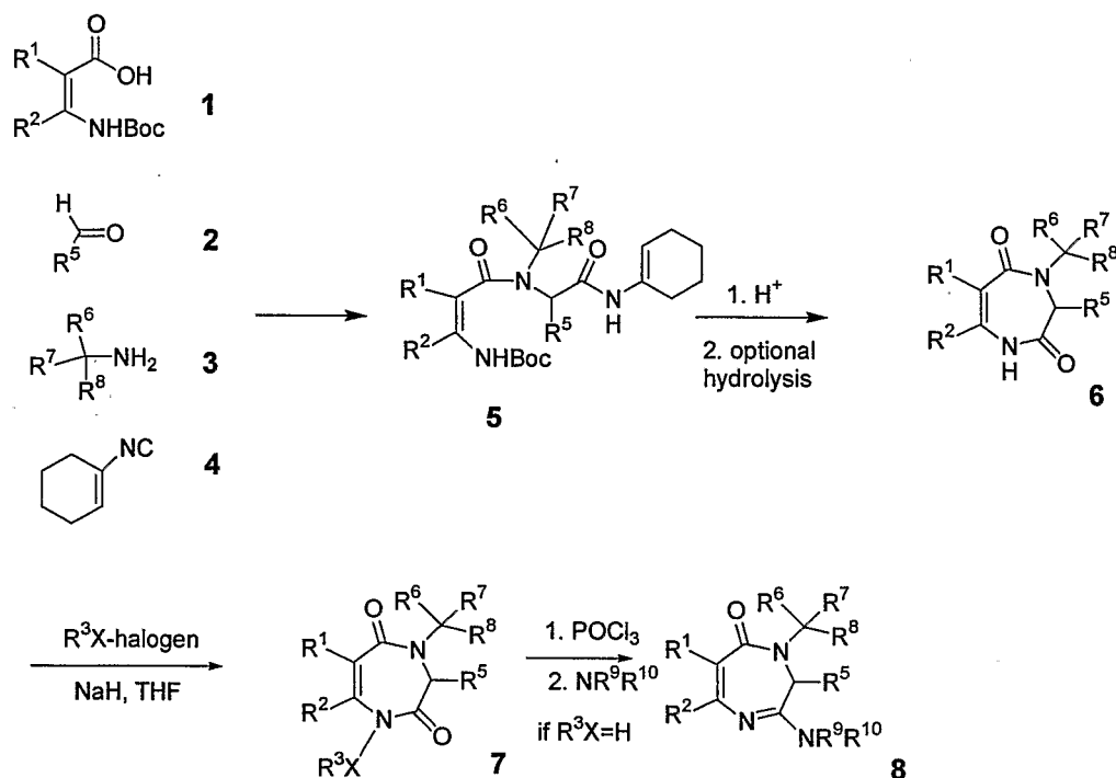
Scheme 1: Conventional Diazepine Synthesis
