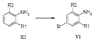
Scheme 7.
