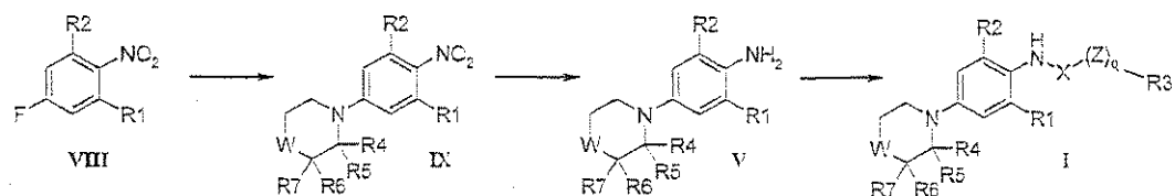
Scheme 4.
