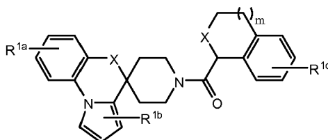
Formula VII
