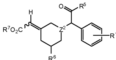
Formula VI
