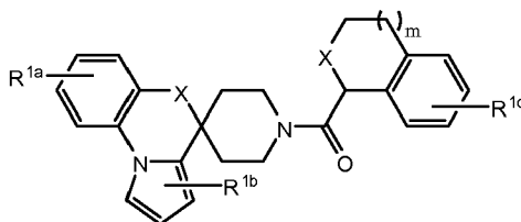
Formula VII
