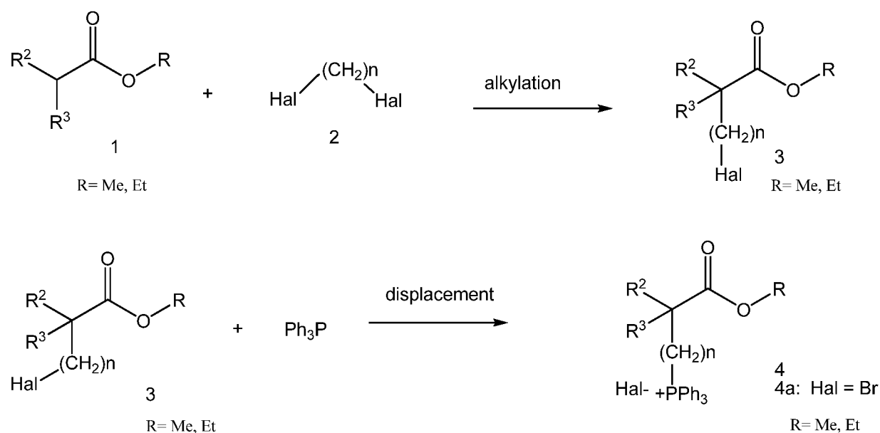
Scheme 1:
