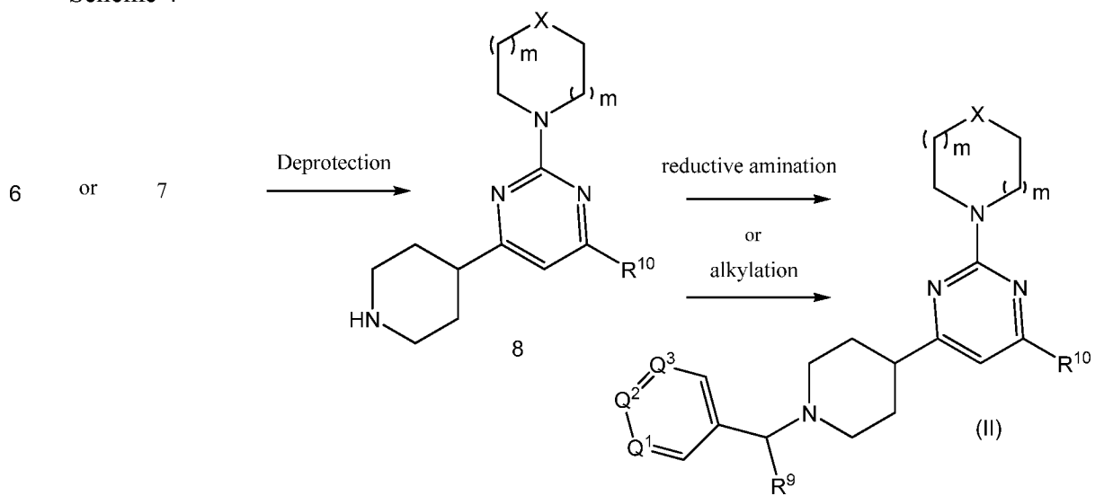
Scheme 4
