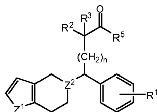
Formula III
