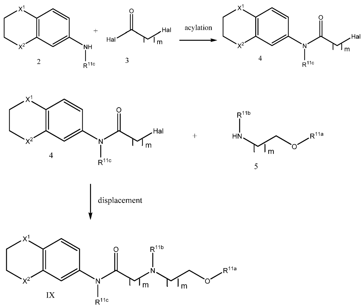
Scheme 2:
