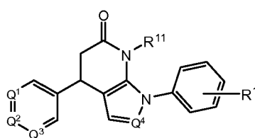
Formula VIII
