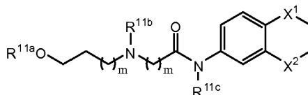
Formula XI
