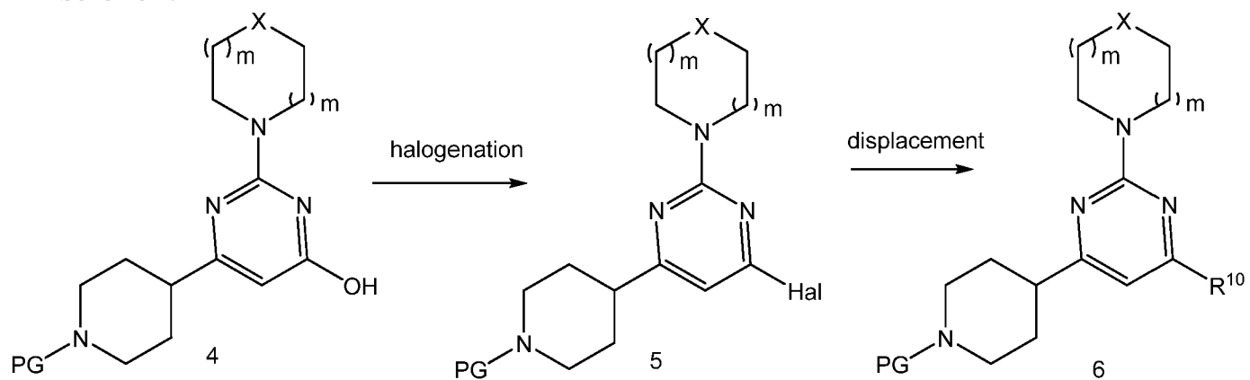
Scheme 2:
