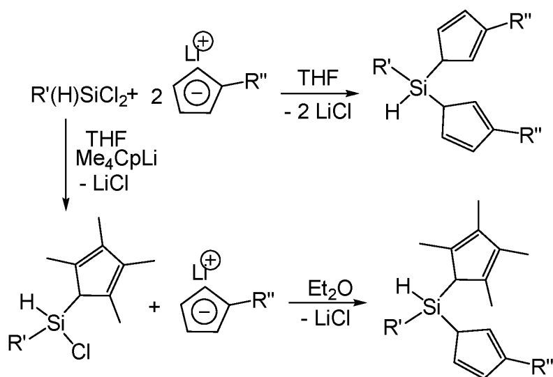
Scheme 1. General synthetic route for Si(H)-bridged cyclopentadienyl ligands (where R' = Me, Ph and R'' = Pr, -CH_2SiMe_3 ).
