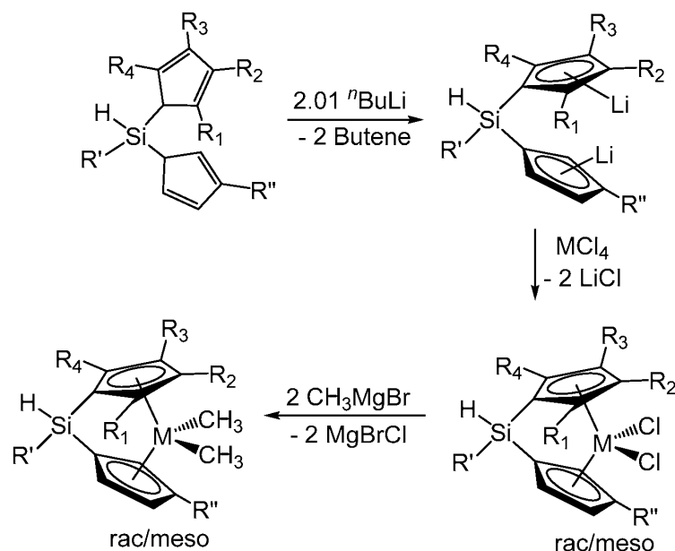
Scheme 2. General synthetic route for Si(H)-bridged metallocenes (where M= Hf, Zr; R'= Me, Ph; R''= n-Pr, -CH 2 SiMe 3 ; R 1 =R 3 =R 4 = Me, H; R 2 = Me, n-Pr, -CH 2 SiMe 3 ).
