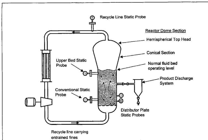
Instrument Locations on Pilot-Scale Reactor
