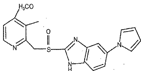
(Ilaprazole)
