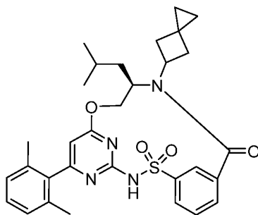
Compound VIII ,
