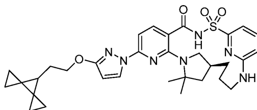
Compound VII ,
