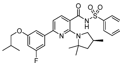
Compound IX ,
