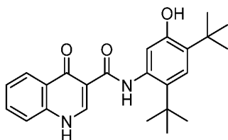
Compound III ,
