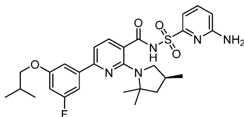
(Compound X).
