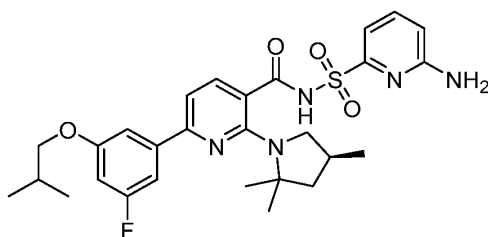
Compound X , and deuterated
