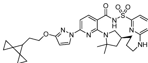
Compound VII ,
