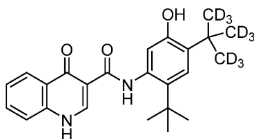
Compound III-d , and deuterated derivatives
