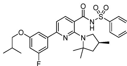
Compound IX ,
