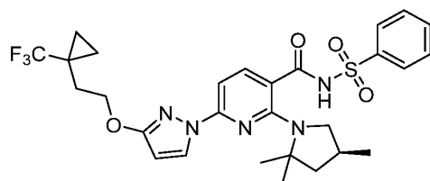
Compound VI ,
