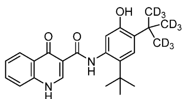
(Compound III-d ).
