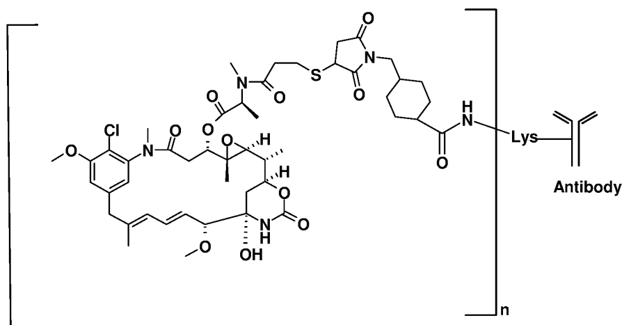
Ab-SMCC-DM1
