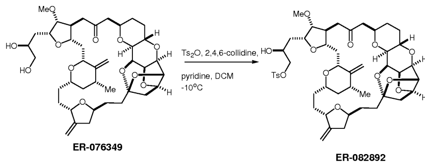
Scheme 8
