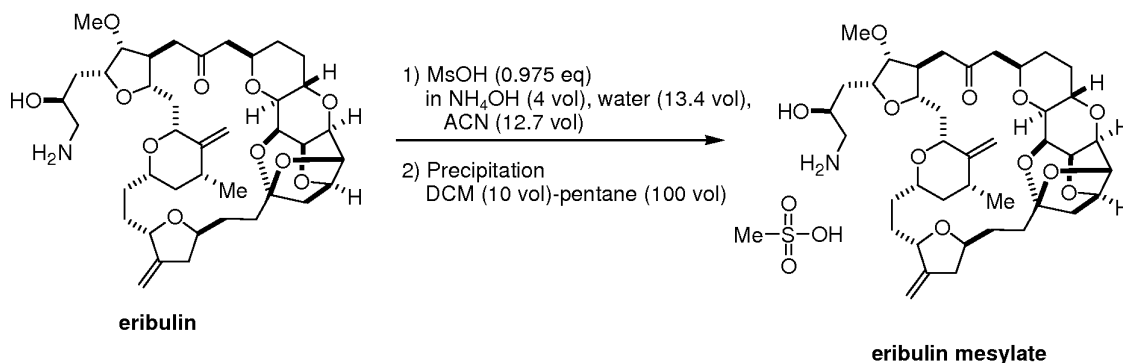
Scheme 13
