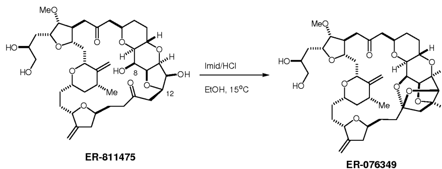
Scheme 6
