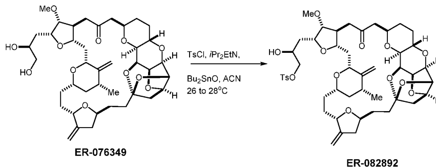
Scheme 10
