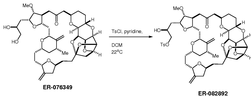
Scheme 7
