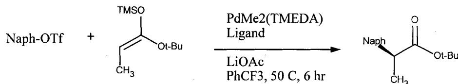
SCHEME I
