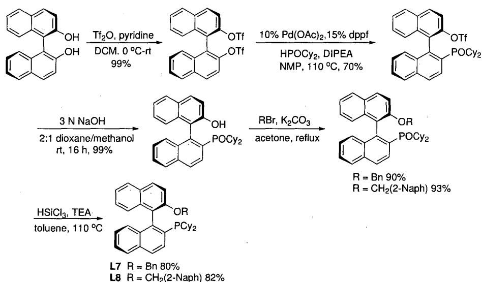
SCHEME V
