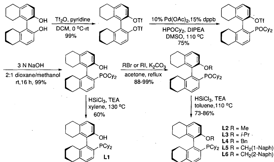
SCHEME IV
