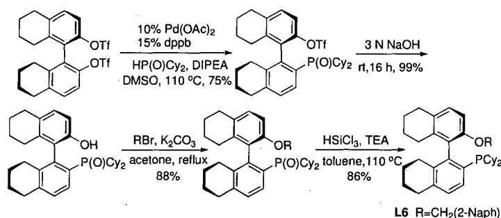
SCHEME II
