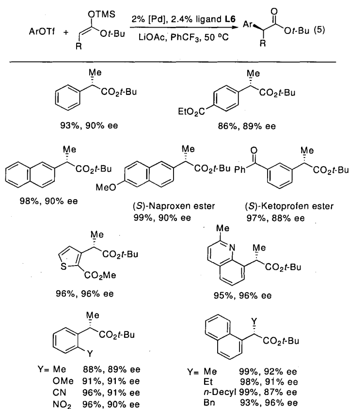
SCHEME III
