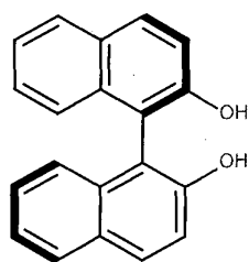
(R)-BINOL
