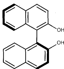
(S)-BINOL
