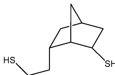
5-(2-mercaptoethyl)-norbornane-3-thiol
