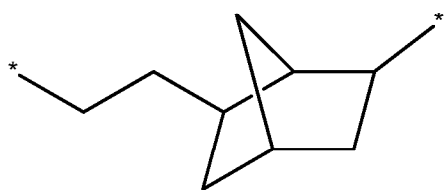
5-(ethyl-2-yl)norborn-3-yl group
