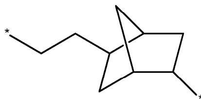
5-(ethyl-2-yl)norborn-2-yl group
