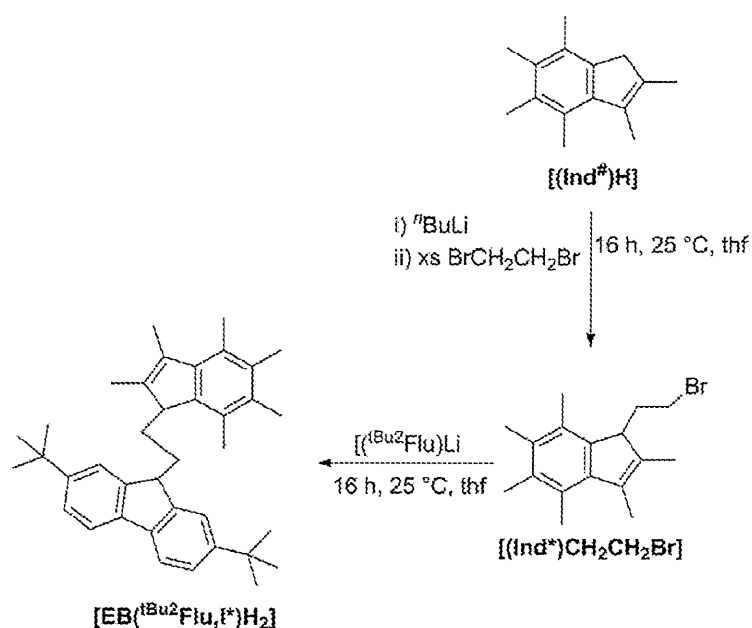
Scheme 1 - Synthesis of [\text{EB}(\text{tBu}_2\text{Flu}, \text{I}^*)\text{H}_2] ethylene-bridged pro-ligand
