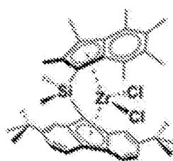
\text{SB}(\text{tBu}_2\text{Flu}, \text{I}^*)\text{ZrCl}_2
