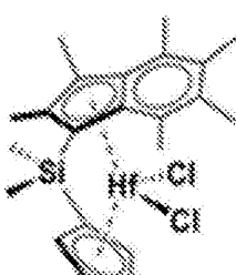
\text{SB}(\text{Cp}, \text{I}^*)\text{HfCl}_2
