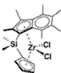
\text{SB}(\text{Cp}, \text{I}^*)\text{ZrCl}_2
