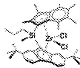
\text{Me,PropSB}(\text{tBu}_2\text{Flu}, \text{I}^*)\text{ZrCl}_2
