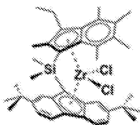
\text{SB}(\text{tBu}_2\text{Flu}, \text{I}^*, 3\text{-ethyl})\text{ZrCl}_2
