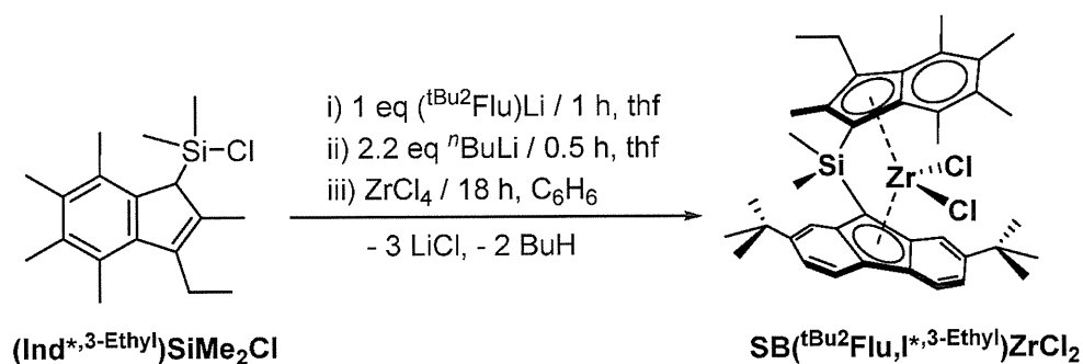
Scheme 6 - synthesis of \text{SB}(\text{tBu}_2\text{Flu}, \text{I}^*, 3\text{-Ethyl})\text{ZrCl}_2 Si-bridged pro-catalyst
