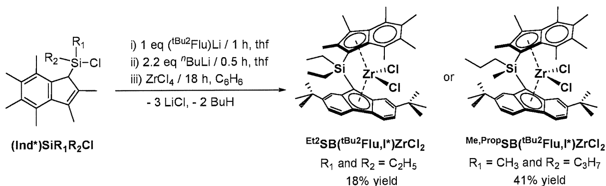
Scheme 5 - synthesis of \text{Et}_2\text{SB}(\text{tBu}_2\text{Flu}, \text{I}^*)\text{ZrCl}_2 and \text{Me,PropSB}(\text{tBu}_2\text{Flu}, \text{I}^*)\text{ZrCl}_2 Si-bridged pro-catalysts
