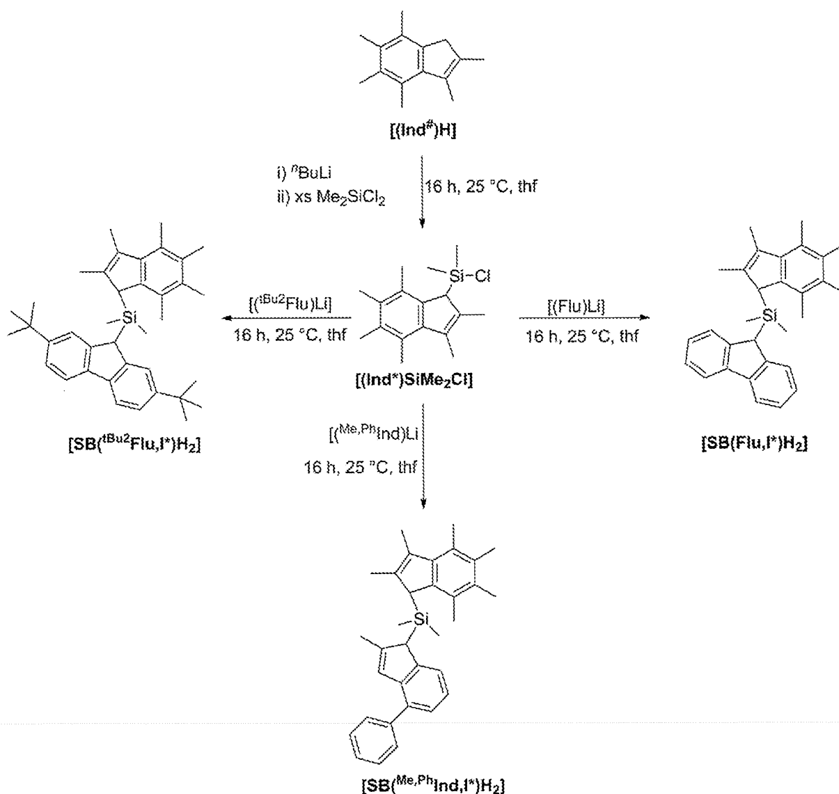
Scheme 3 - Synthesis of [\text{SB}(\text{tBu}_2\text{Flu},\text{I}^*)\text{H}_2] , [\text{SB}(\text{Flu},\text{I}^*)\text{H}_2] and [\text{SB}(\text{Me,PhInd},\text{I}^*)\text{H}_2] Si-bridged pro-ligands
