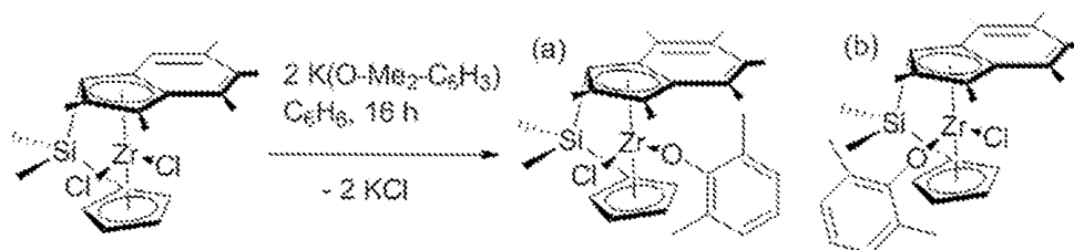
Scheme 9 - synthesis of \text{SB}(\text{Cp}, \text{I}^*)\text{ZrCl}(\text{O}-2,6\text{-Me}_2\text{-C}_6\text{H}_3) Si-bridged pro-catalysts
