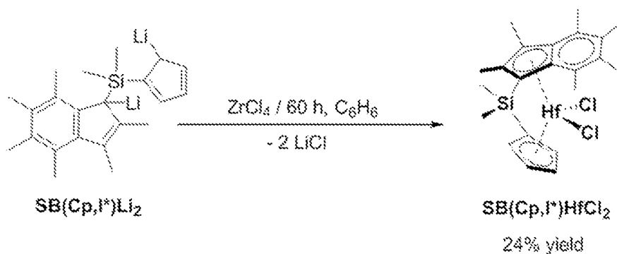
Scheme 8 - synthesis of \text{SB}(\text{Cp},\text{I}^*)\text{HfCl}_2 Si-bridged pro-catalyst
