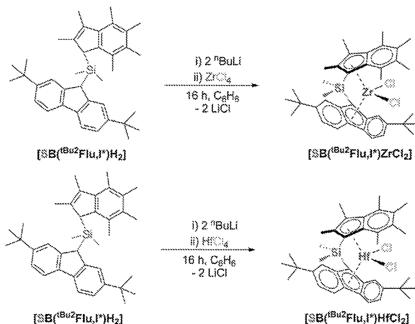
Scheme 4 - synthesis of [\text{SB}(\text{tBu}_2\text{Flu}, \text{I}^*)\text{ZrCl}_2] and [\text{SB}(\text{tBu}_2\text{Flu}, \text{I}^*)\text{HfCl}_2] Si-bridged pro-catalysts
