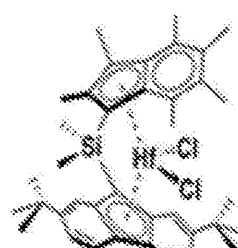
\text{SB}(\text{tBu}_2\text{Flu}, \text{I}^*)\text{HfCl}_2
