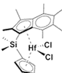
SB(Cp, I*)HfCl 2
