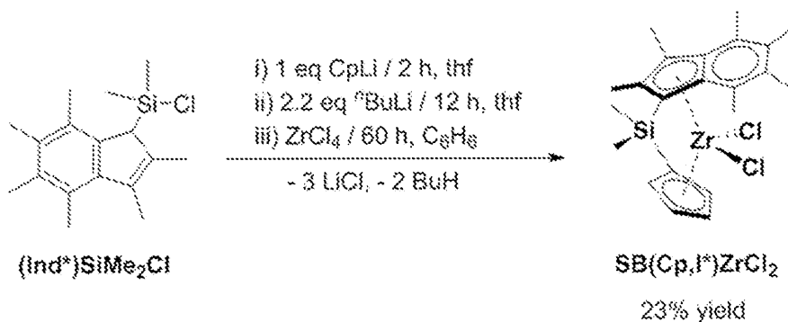
Scheme 7 - synthesis of \text{SB}(\text{Cp},\text{I}^*)\text{ZrCl}_2 Si-bridged pro-catalyst
