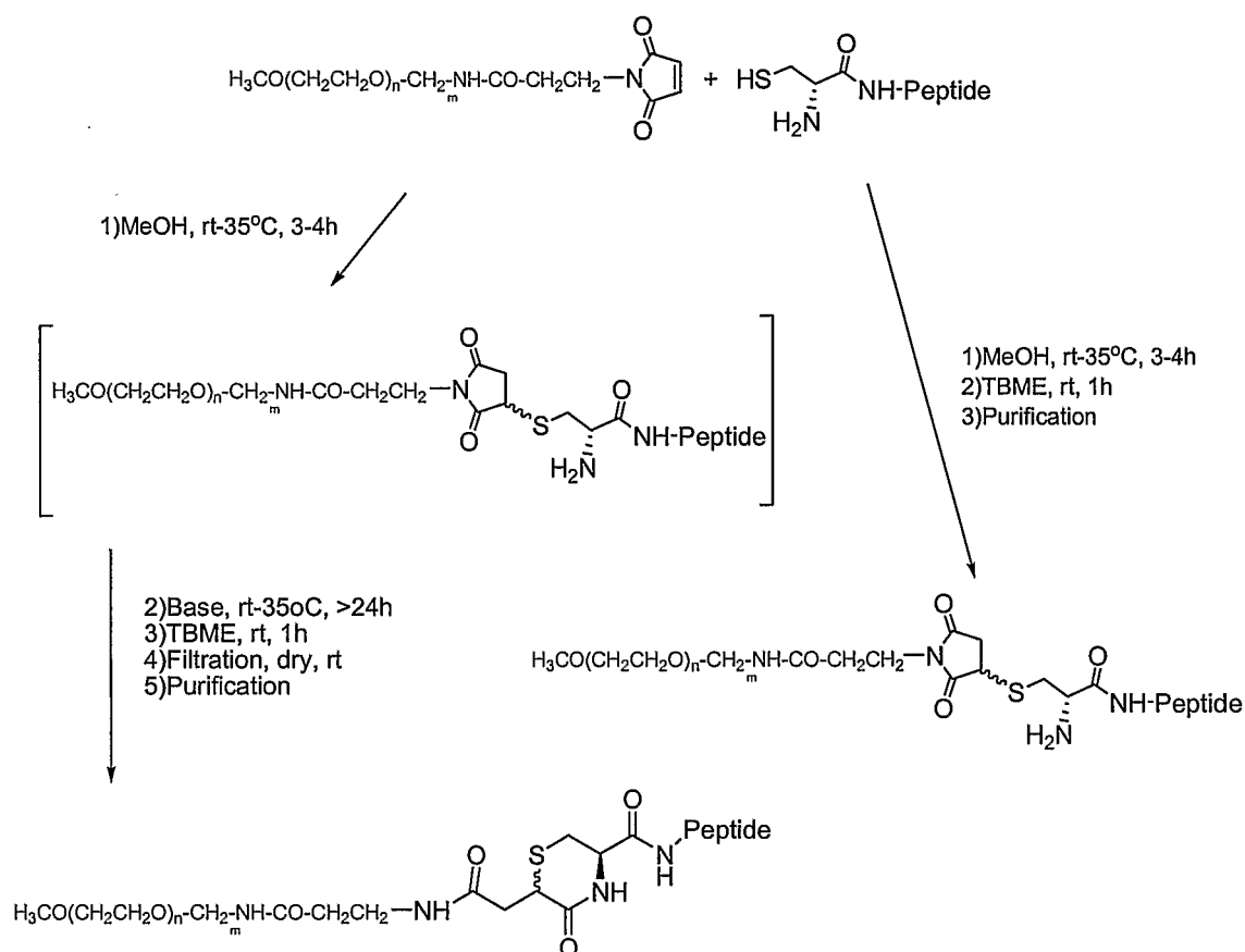
Scheme 4
