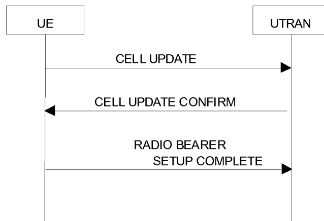
Figure 8.3.1-6a: Cell update procedure with radio bearer setup
