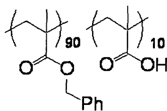
Resin (D-2) Mw 14,000; Mn 8,000
