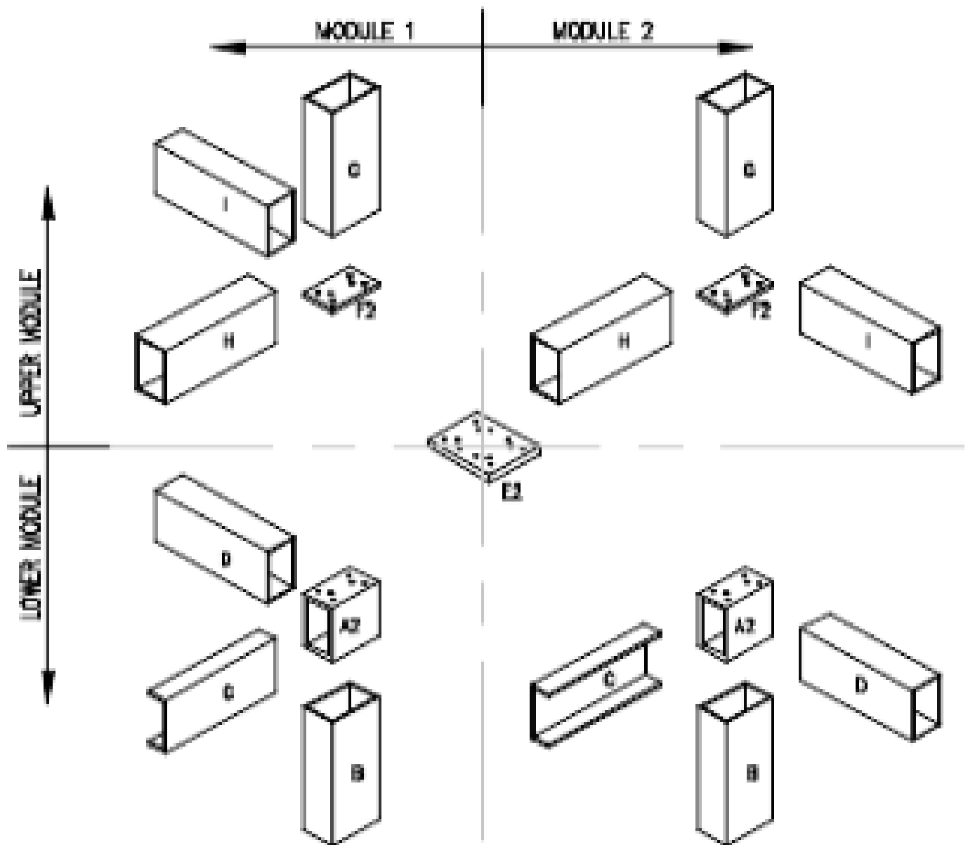
EXPLODED VIEW OF TYPE 2 COLUMN SPLICE JOINT
