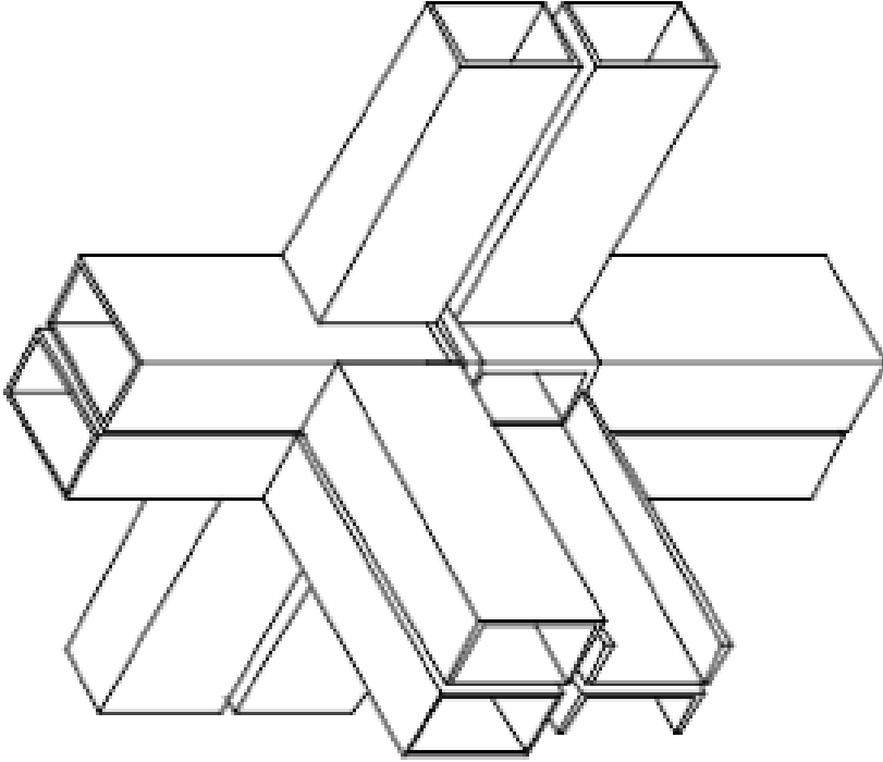
ISOMETRIC VIEW OF TYPE 2 COLUMN SPLICE JOINT
