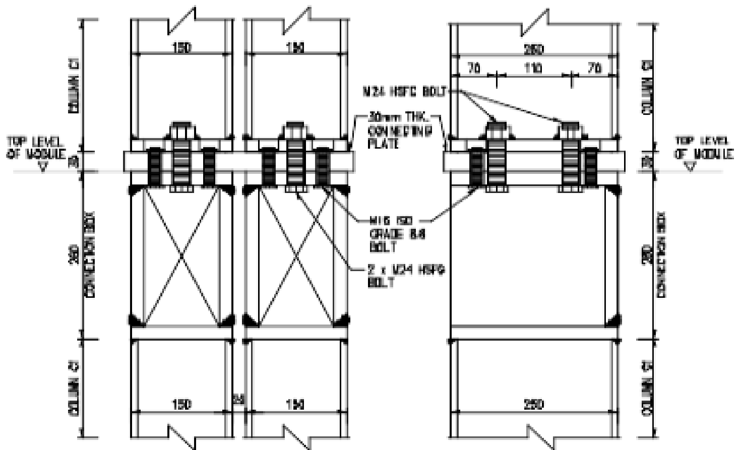
TYPE 2 COLUMN SPLICE
