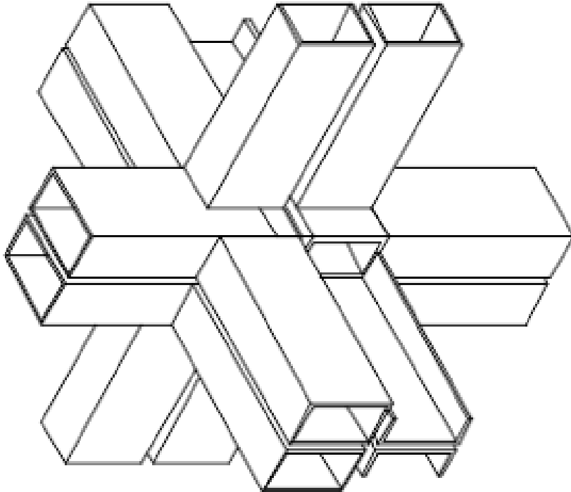
ISOMETRIC VIEW OF TYPE 1 COLUMN SPLICE JOINT
