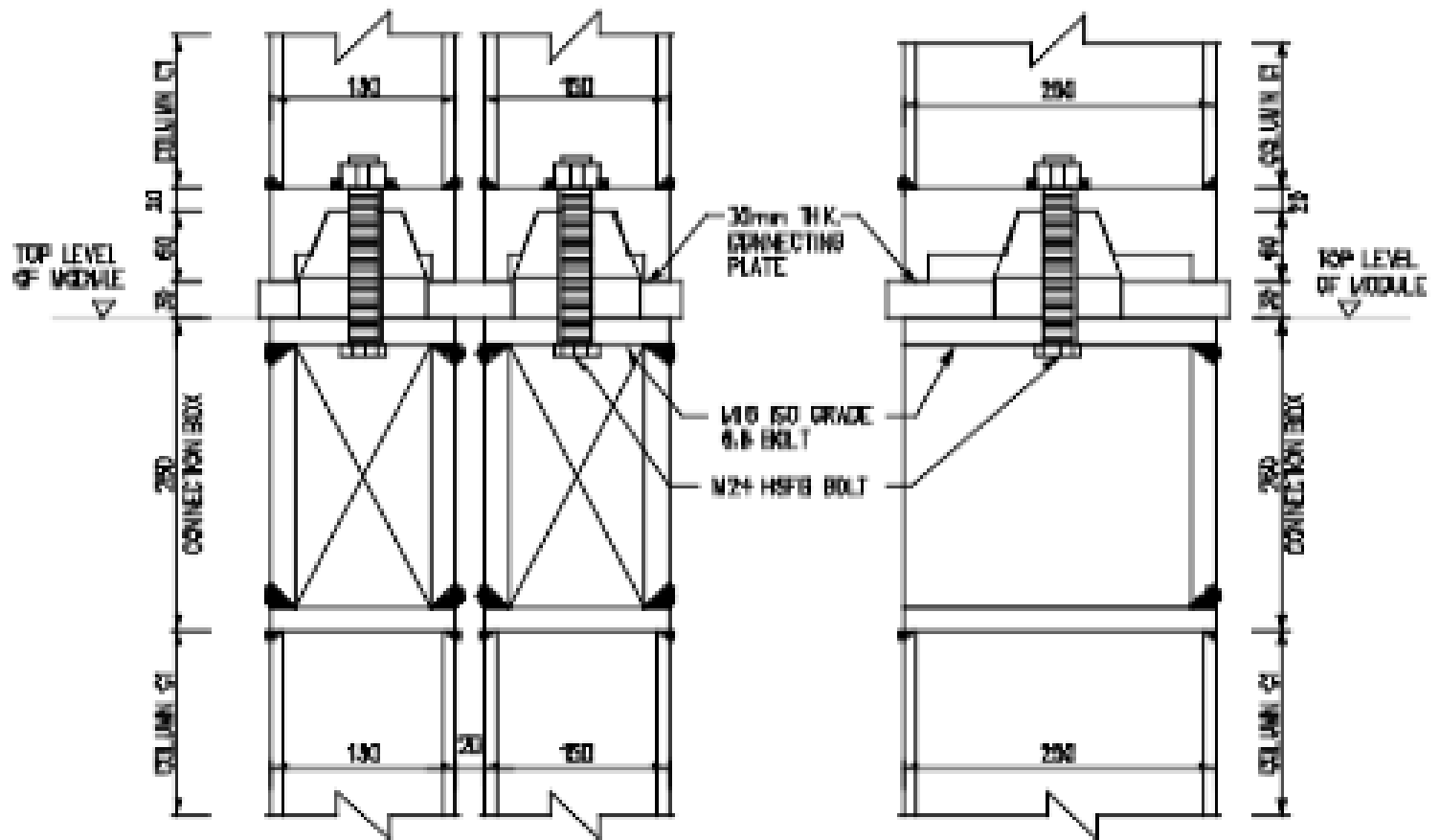
TYPE 1 COLUMN SPLICE
