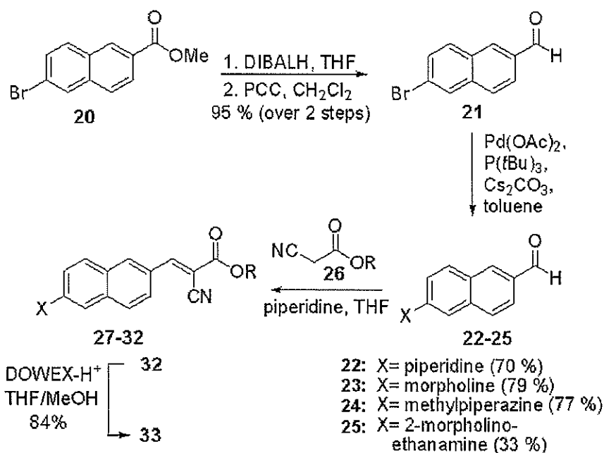
Scheme 5. General strategy for the synthesis of probes 27-33
