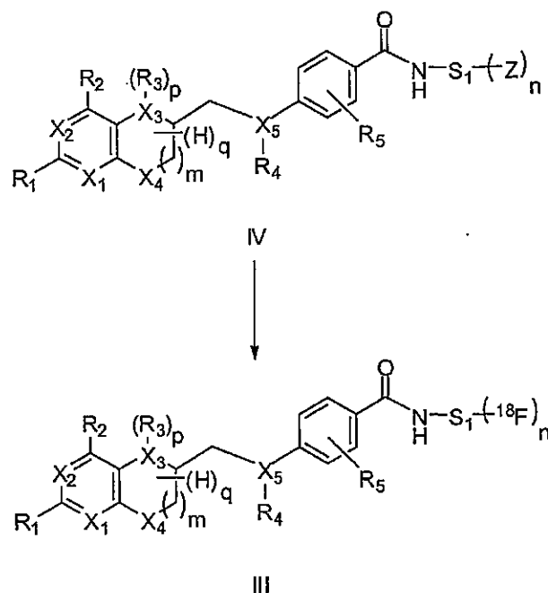
Scheme 1. Synthesis scheme
