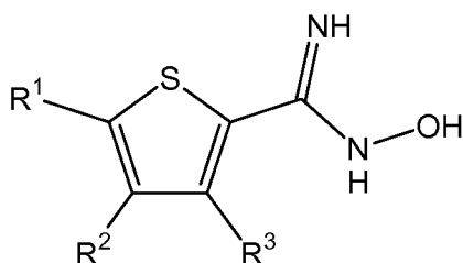
Structure 11
