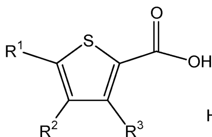
Structure 3
