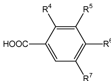
Structure 12
