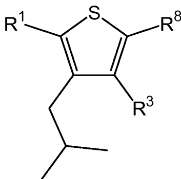
Formula (II)
