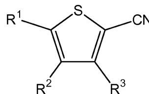
Structure 14
