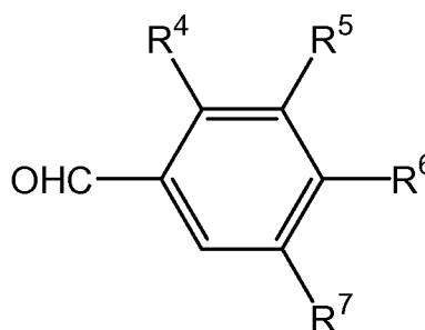
Structure 5
