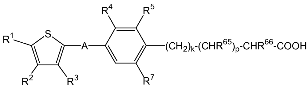
Formula (III)
