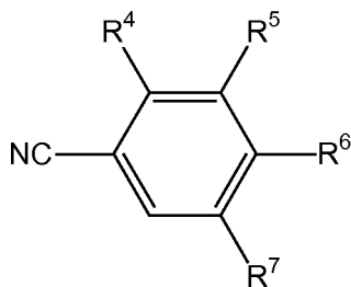
Structure 13
