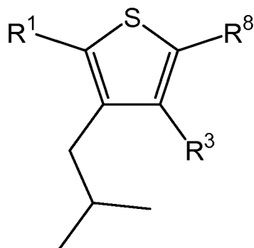
Formula (II)
