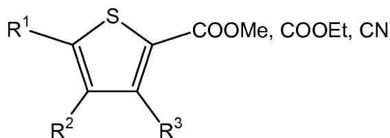
Structure 15
