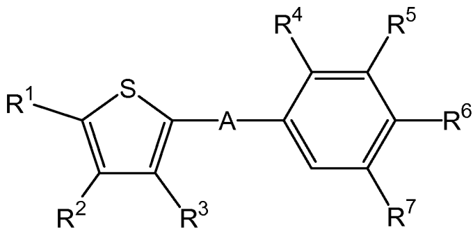
Formula (I)
