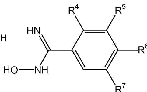
Structure 10
