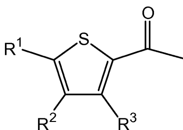
Structure 4
