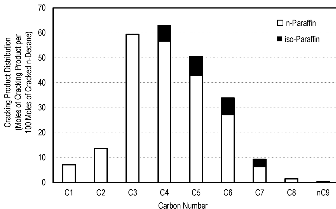
FIG. 11 Cracking Product Distribution at 39.1 mol.% of Cracking Yield
