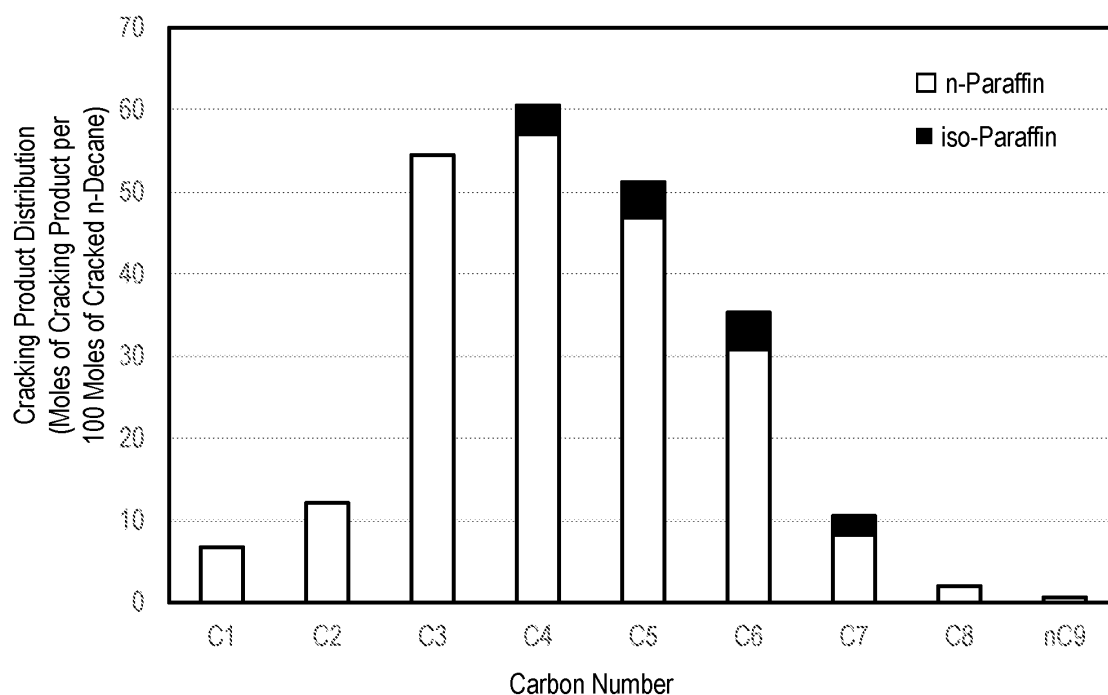
FIG. 7 Cracking Product Distribution at 10.8 mol.% of Cracking Yield
