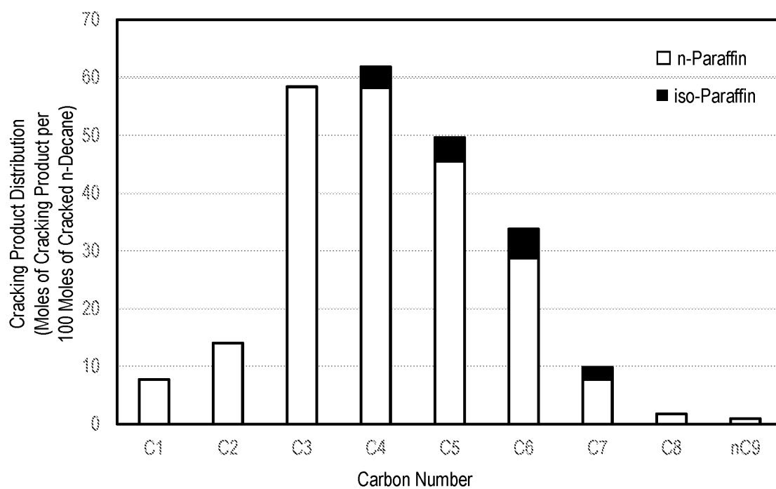
FIG. 6 Cracking Product Distribution at 5.8 mol.% of Cracking Yield
