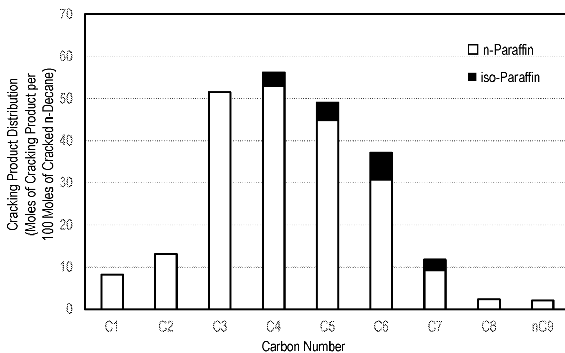
FIG. 5 Cracking Product Distribution at 2.2 mol.% of Cracking Yield
