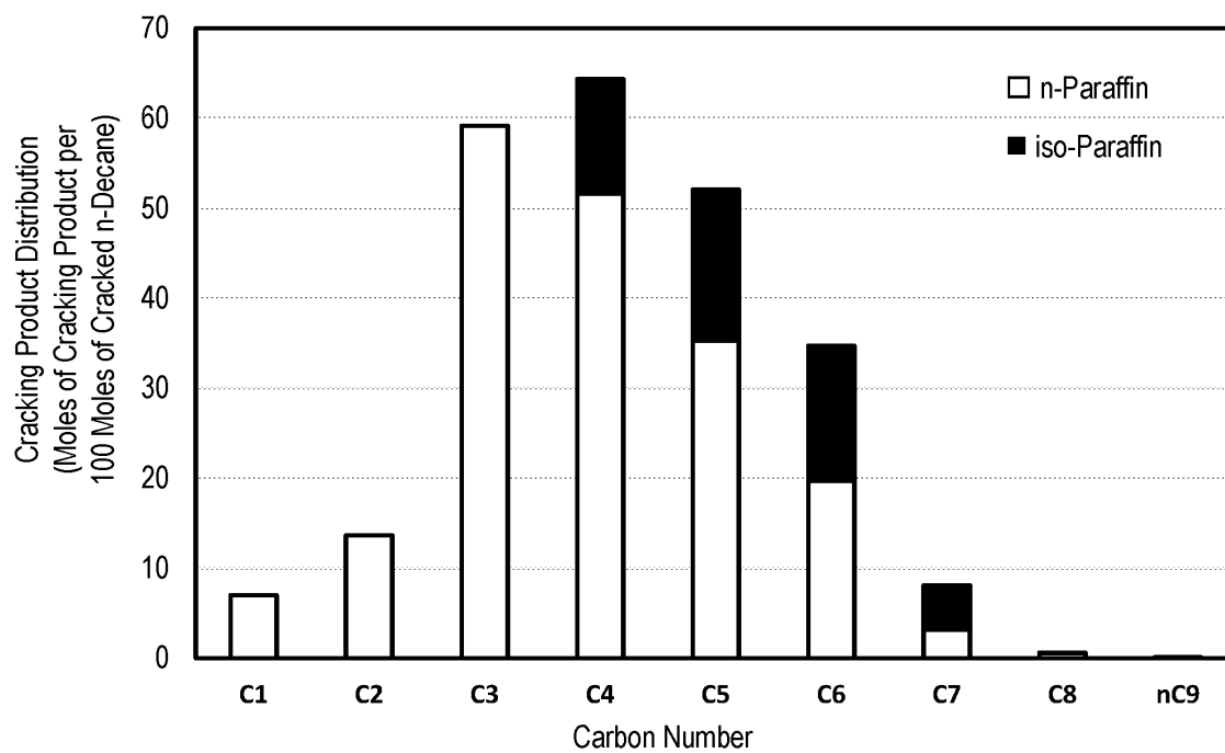
FIG. 13 Cracking Product Distribution at 65.9 mol.% of Cracking Yield
