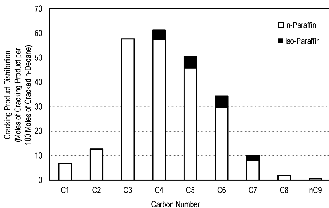
FIG. 8 Cracking Product Distribution at 14.6 mol.% of Cracking Yield
