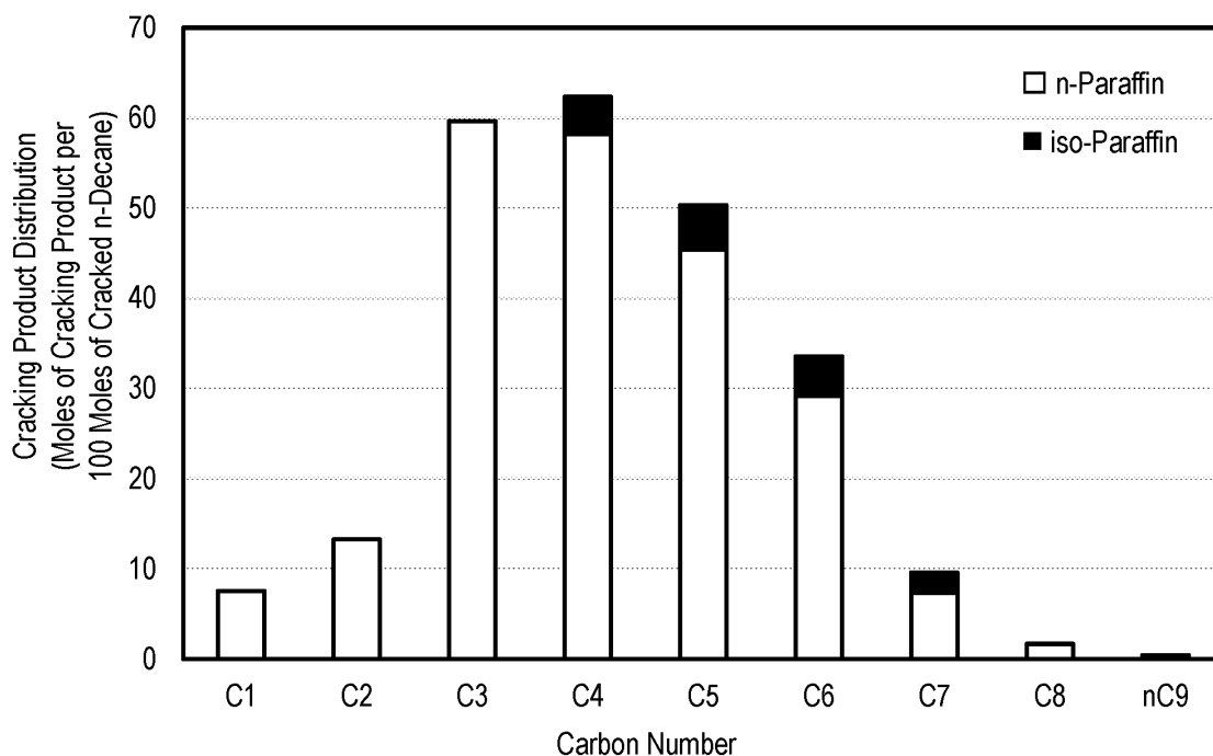
FIG. 9 Cracking Product Distribution at 20.6 mol.% of Cracking Yield
