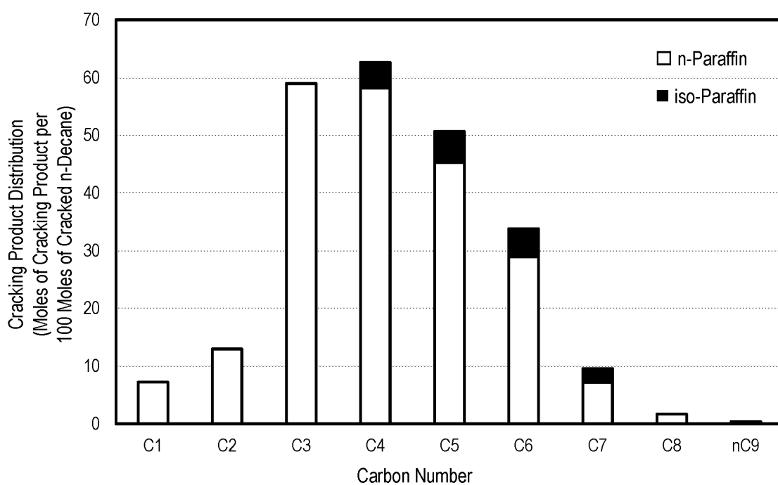
FIG. 10 Cracking Product Distribution at 28.2 mol.% of Cracking Yield
