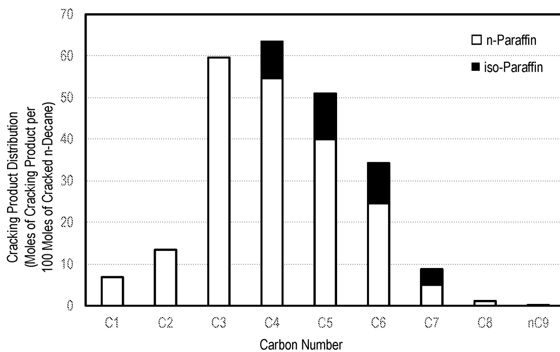
FIG. 12 Cracking Product Distribution at 50.3 mol.% of Cracking Yield
