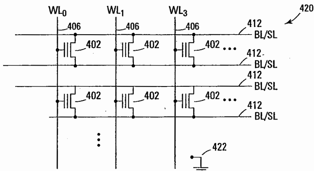
Fig. 4C Prior Art
