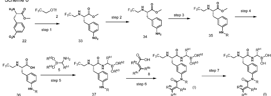
Scheme 7
