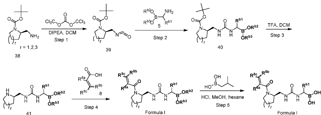
Scheme 7
