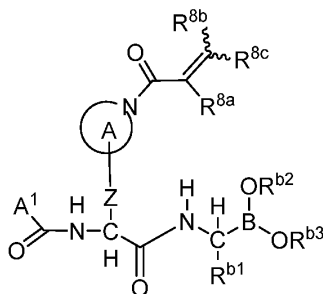
Formula I(c)
