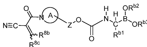
Formula I(a)
