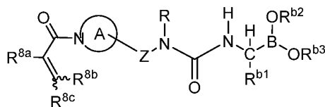
Formula I(e)
