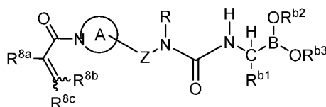
Formula I(b)
