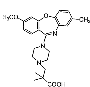
Compound 87
