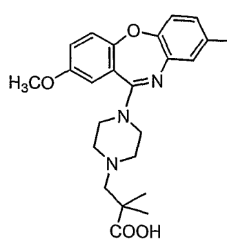
Compound 54
