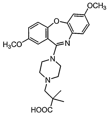
Compound 35
