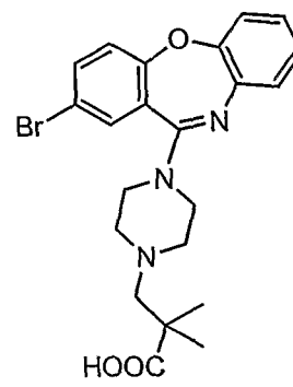
Compound 8
