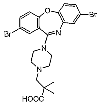
Compound 18
