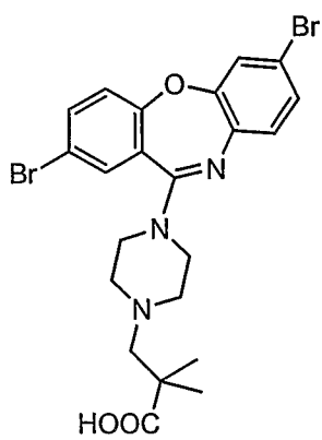
Compound 29
