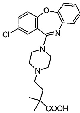
Compound 6
