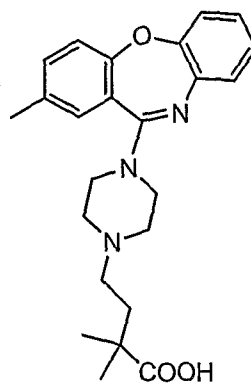
Compound 11
