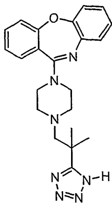
Compound 41
