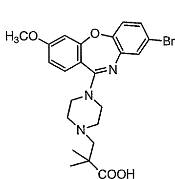
Compound 86
