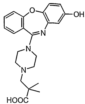
Compound 24
