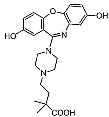
Compound 66
