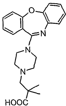
Compound 1
