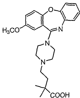
Compound 13
