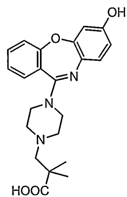
Compound 37
