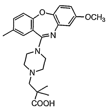
Compound 56
