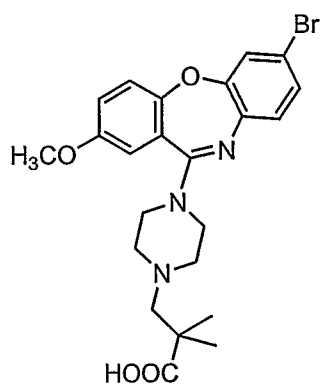
Compound 72
