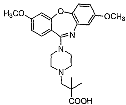
Compound 42
