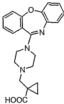
Compound 2
