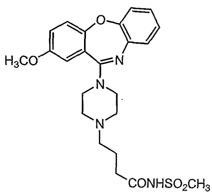
Compound 77
