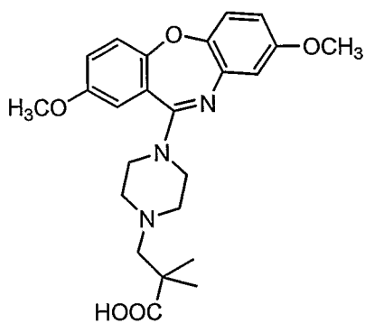
Compound 23
