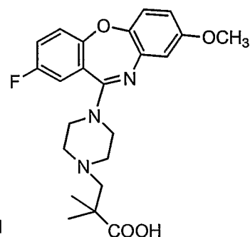
Compound 85
