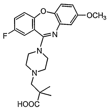
Compound 22
