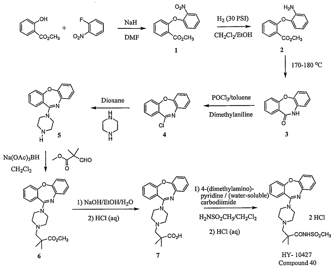
Scheme I
