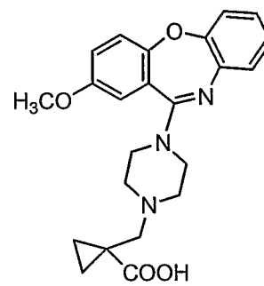
Compound 63
