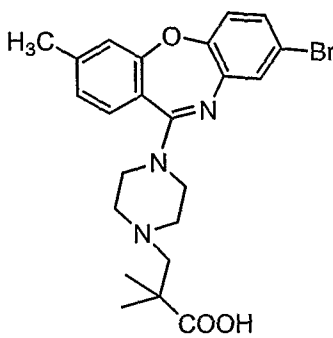
Compound 44
