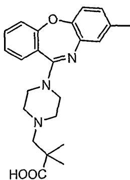
Compound 19
