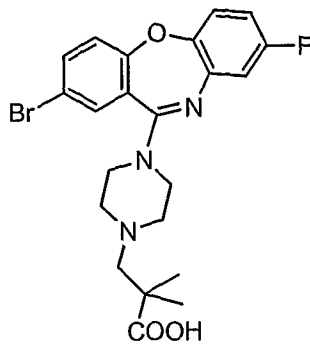
Compound 47
