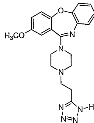
Compound 74
