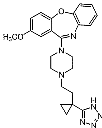
Compound 82
