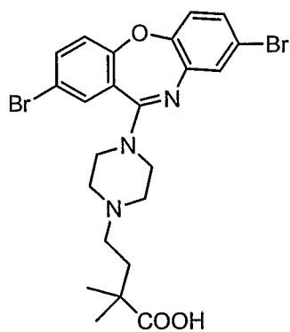
Compound 64
