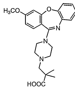
Compound 39
