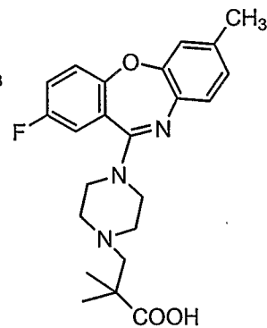
Compound 88
