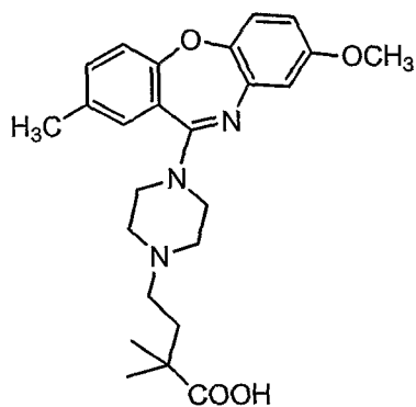
Compound 43
