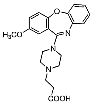
Compound 61
