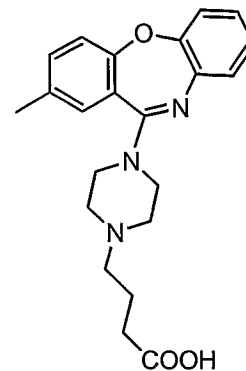
Compound 60
