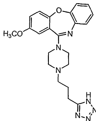
Compound 76
