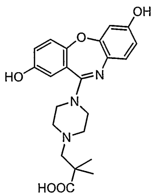
Compound 38
