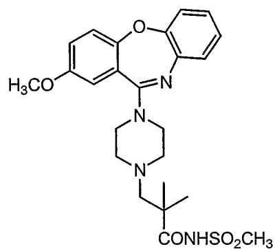
Compound 71
