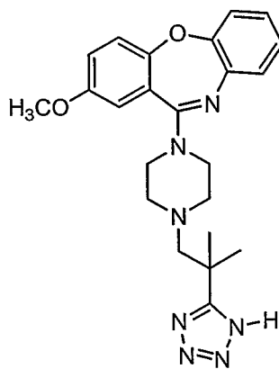
Compound 70
