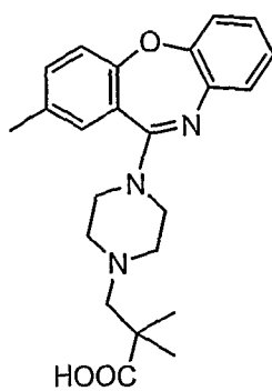
Compound 10
