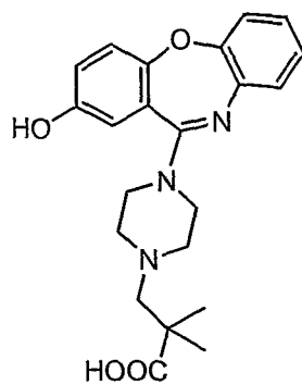
Compound 14
