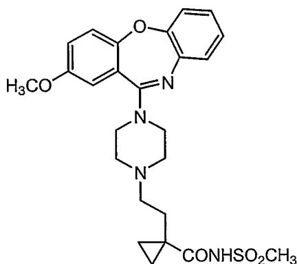
Compound 83
