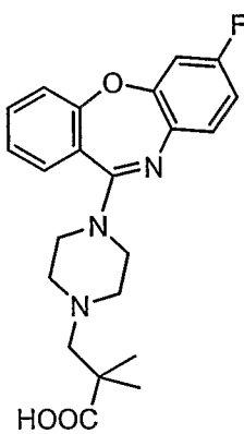
Compound 26
