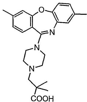
Compound 52
