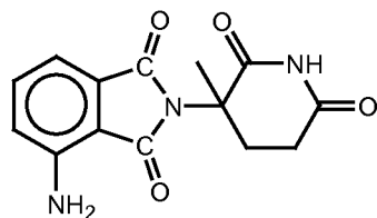
1,3-dioxo-2-(3-methyl-2,6-dioxopiperidin-3-yl)-4-aminoisoindole,
