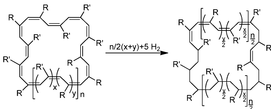
Scheme 3
