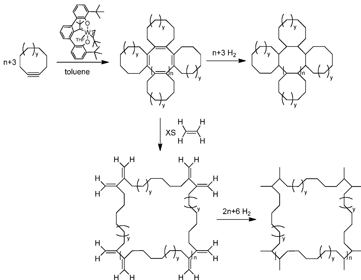
Scheme 4
