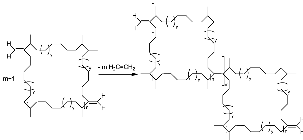
Scheme 5
