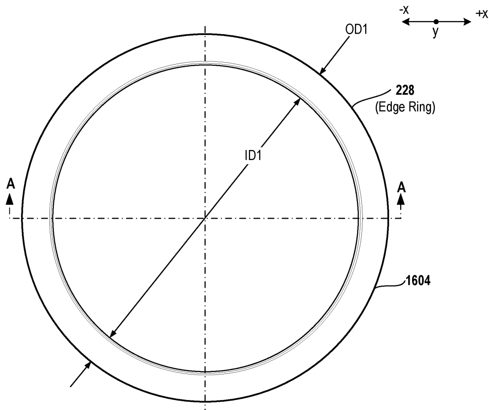
FIG. 8B (Top View)
