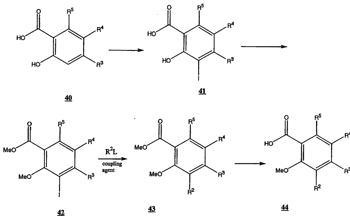
Scheme X:
