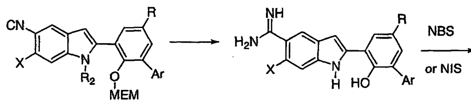
Scheme LXXIII
