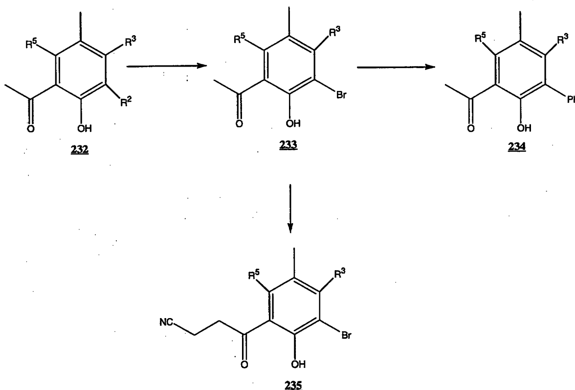
Scheme LVIII
