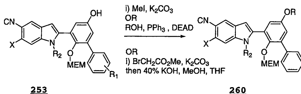
Scheme LXX
