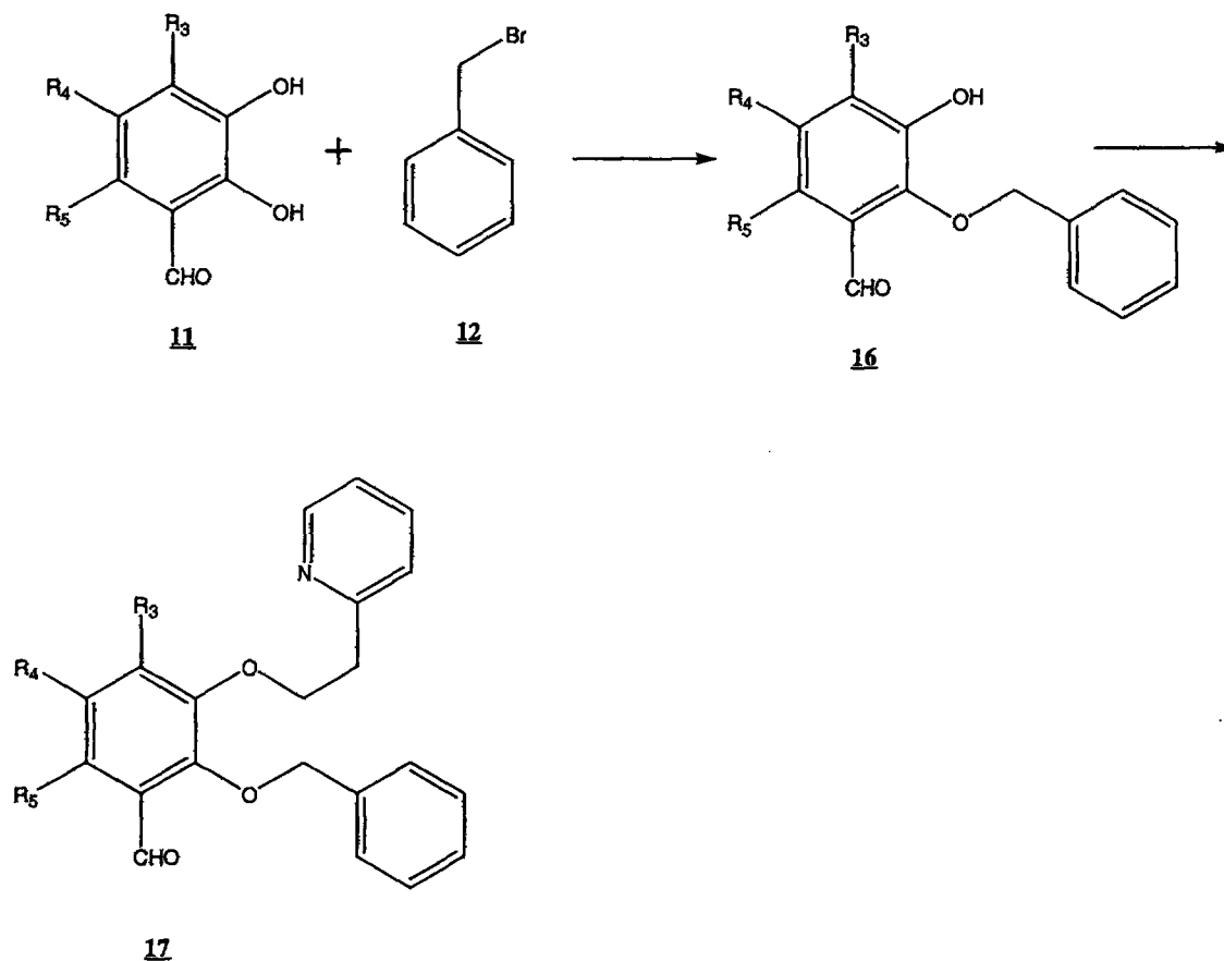
Scheme VII
