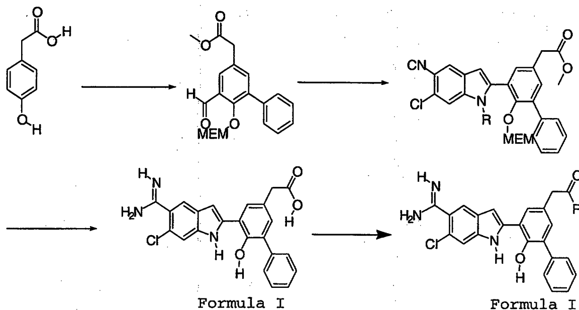
Scheme LXXI
