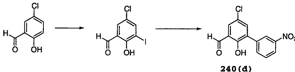
Scheme LX(4)
