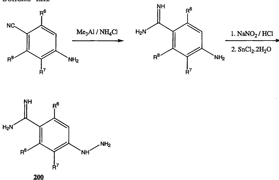
Scheme LXI
