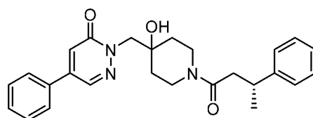
Example 38: (R)-4-(2-Cyanophenyl)-1-((4-hydroxy-1-(3-phenylbutanoyl)piperidin-4-yl)methyl)-N-isopropyl-N-methyl-6-oxo-1,6-dihydropyridine-3-carboxamide
