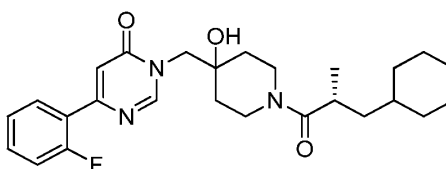
Example 40: 3-((1-(2-(Cyclohexylmethyl)butanoyl)-4-hydroxypiperidin-4-yl)methyl)-6-(2-fluorophenyl)pyrimidin-4(3H)-one
