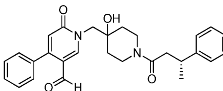
Example 45: (R)-1-((4-Hydroxy-1-(3-phenylbutanoyl)piperidin-4-yl)methyl)-6-oxo-4-phenyl-1,6-dihydropyridine-3-carbaldehyde
