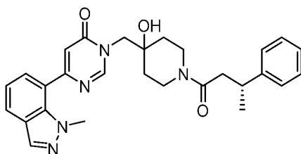
Example 17: (R)-3-((4-Hydroxy-1-(3-phenylbutanoyl)piperidin-4-yl)methyl)-6-(2-methoxyphenyl)pyrimidin-4(3H)-one
