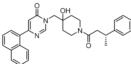
Example 20: (R)-3-((4-Hydroxy-1-(3-phenylbutanoyl)piperidin-4-yl)methyl)-6-(naphthalen-1-yl)pyrimidin-4(3H)-one
