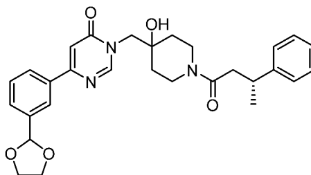
Example 22: (R)-3-((4-Hydroxy-1-(3-phenylbutanoyl)piperidin-4-yl)methyl)-6-(thiophen-3-yl)pyrimidin-4(3H)-one
