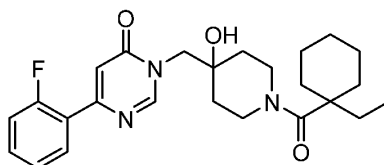
Example 25: 3-((1-(2-(Cyclohexylmethyl)-3-methylbutanoyl)-4-hydroxy-3,3-dimethylpiperidin-4-yl)methyl)-6-(2-fluorophenyl)pyrimidin-4(3H)-one
