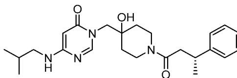
10 Example 35: (R)-3-((4-Hydroxy-1-(3-phenylbutanoyl)piperidin-4-yl)methyl)-6-(isobutylamino)pyrimidin-4(3H)-one
