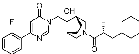
Example 32: (R)-6-(2-Fluorophenyl)-3-((4-hydroxy-1-(3-phenylbutanoyl)piperidin-4-yl)methyl)pyrimidin-4(3H)-one
