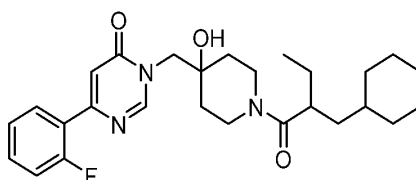
Example 40: 3-((1-(2-(Cyclohexylmethyl)butanoyl)-4-hydroxypiperidin-4-yl)methyl)-6-(2-fluorophenyl)pyrimidin-4(3H)-one
