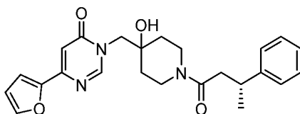
Example 27: (R)-1-((4-Hydroxy-1-(3-phenylbutanoyl)piperidin-4-yl)methyl)-4-phenylpyridin-2(1H)-one
