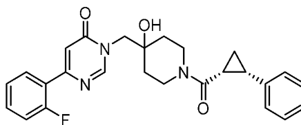
Example 42: 6-(2-Fluorophenyl)-3-((4-hydroxy-1-(1-methylcyclohexanecarbonyl)piperidin-4-yl)methyl)pyrimidin-4(3H)-one
