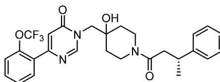
10 Example 30: (R)-3-((4-Hydroxy-1-(3-phenylbutanoyl)piperidin-4-yl)methyl)-6-(2-(trifluoromethoxy)phenyl)pyrimidin-4(3H)-one
