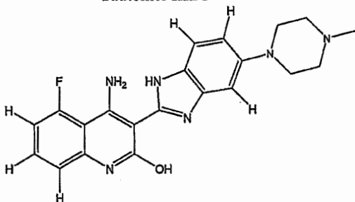
Tautomer IIIBc
