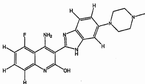
Tautomer IIIBa
