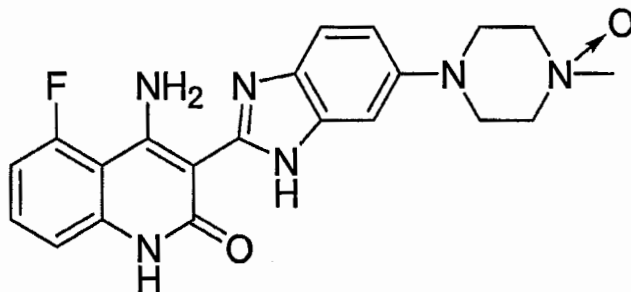
Compound 2
