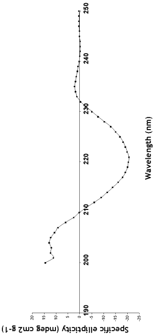
rhTRAIL95-281 protein
