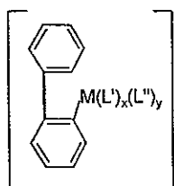
Structure IV
