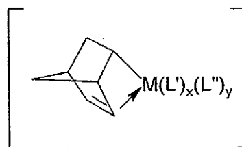
Structure II
