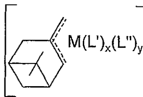
Structure VIb
