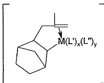
Structure III
