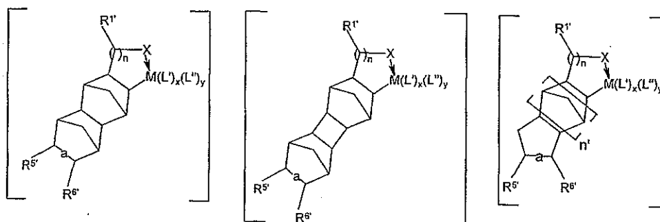
Structure Vh
