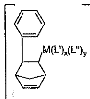
Structure IVb
