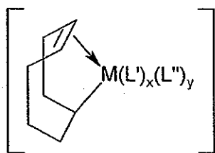
Structure I
