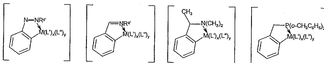
Structure Vd
