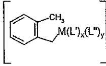
Structure IVa
