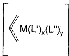
Structure VIa
