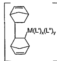
Structure IVc
