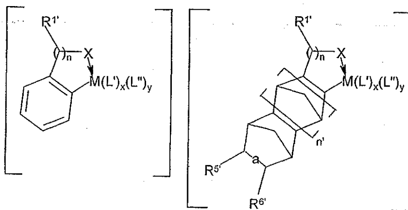
Structure Vb
