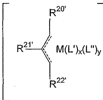
Structure VI
