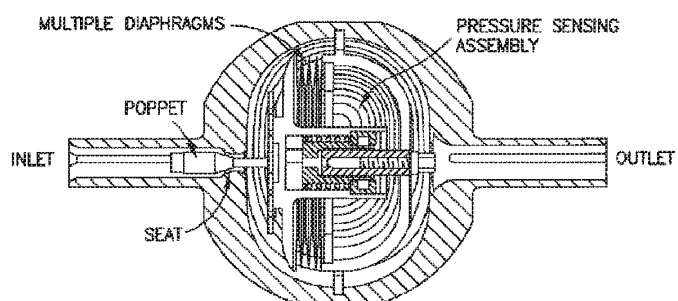
FIG. 4 PRIOR ART
