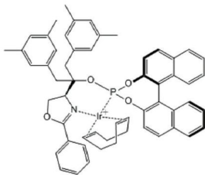
<Compound 3a-1>
