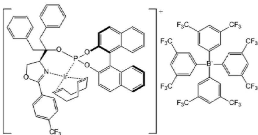
<Compound 5a-7>
