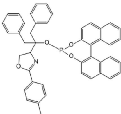
<Compound 1-6>
