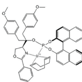
<Compound 3a-2>
