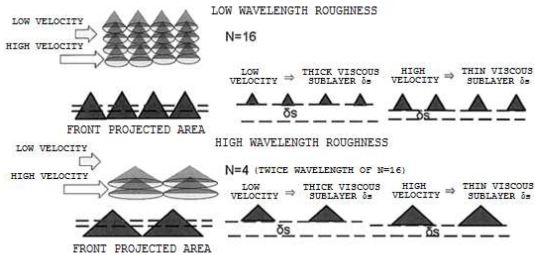
FIG. 3 RELATIONSHIP BETWEEN FRICTION INCREASE RATIO FIR (%) AND A = (R_a - \delta_s)/R_{Sm}
