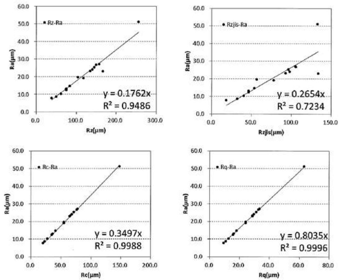
FIG. 6 CORRELATIONS OF R_a WITH PARAMETERS
