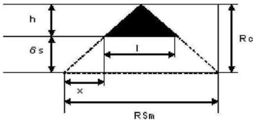
FIG. 4 CALCULATION OF PROMINENT PEAK PROJECTED AREA A FROM VISCOUS SUBLAYER \delta_s USING R_c
