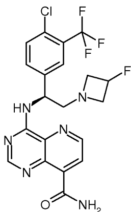
4-[(S)-1-(4-Chloro-3-trifluoromethyl-phenyl)-2-(3-fluoro-azetidin-1-yl)-ethylamino]-pyrido[3,2-d]pyrimidine-8-carboxylic acid amide ( 69 )
