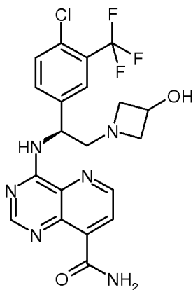
4-[(S)-1-(4-Chloro-3-trifluoromethyl-phenyl)-2-(3-hydroxy-azetidin-1-yl)-ethylamino]-pyrido[3,2-d]pyrimidine-8-carboxylic acid amide ( 70 )
