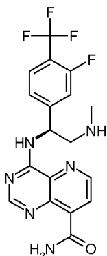
4-[(S)-1-(3-Fluoro-4-trifluoromethyl-phenyl)-2-methylamino-ethylamino]-pyrido[3,2-d]pyrimidine-8-carboxylic acid amide (26)
