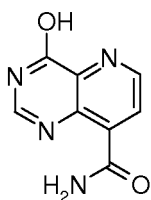
4-hydroxypyrido[3,2-d]pyrimidine-8-carboxamide (G) (Scheme 6)
