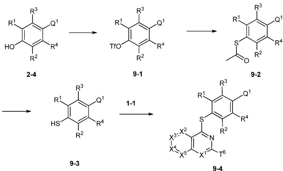
Scheme 9
