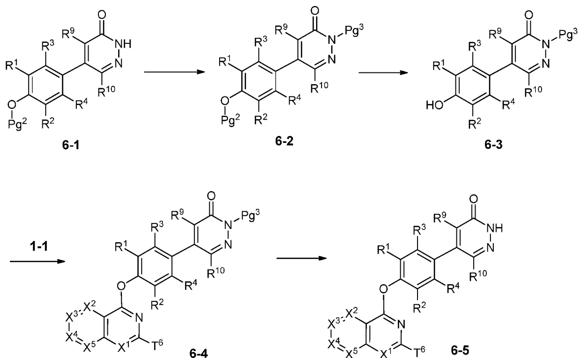
Scheme 6
