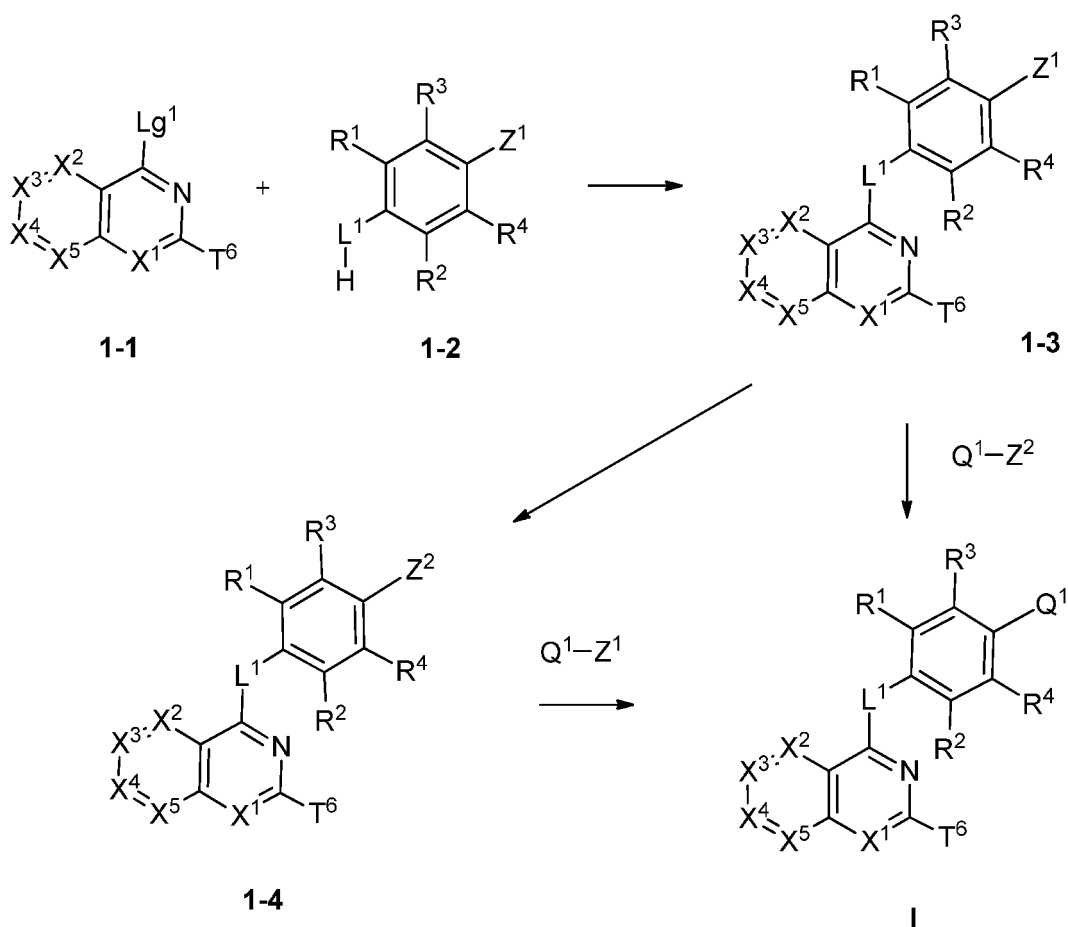
Scheme 1
