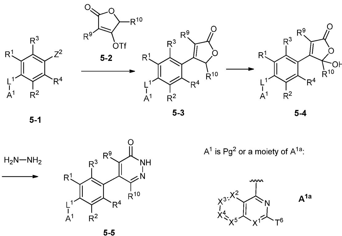
Scheme 5
