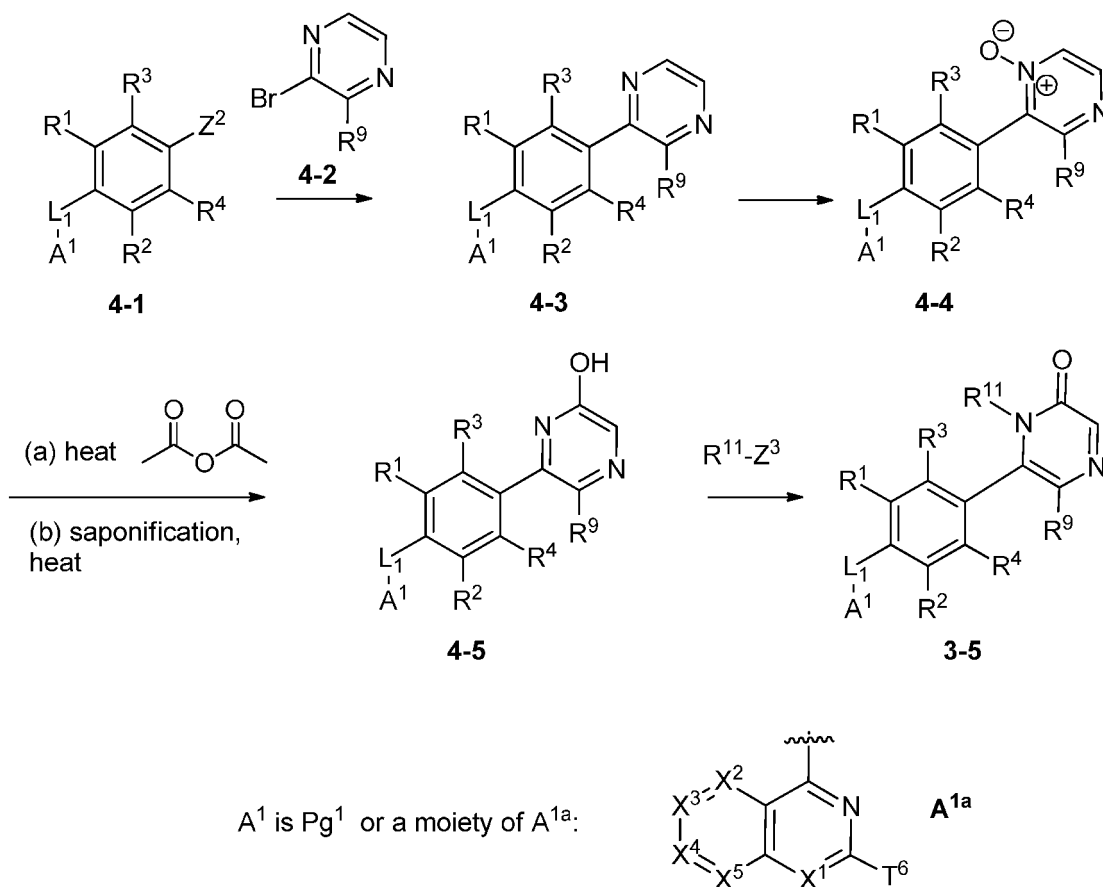
Scheme 4
