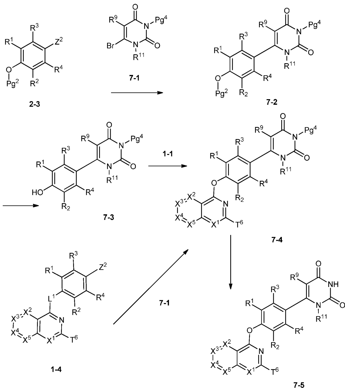
Scheme 7
