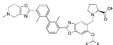
Compound 314
