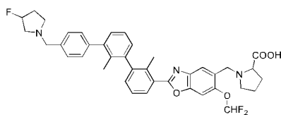
Compound 242
