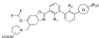
Formula (IV)
