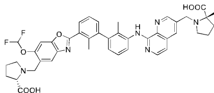
Compound 171
