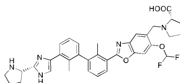
Compound 247
