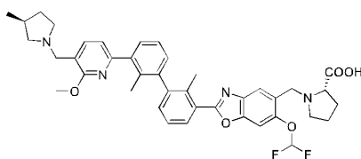
Compound 246
