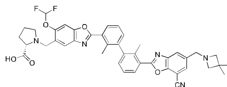
Compound 103
