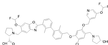
Compound 208
