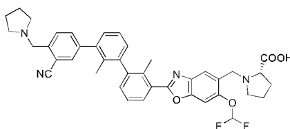
Compound 245
