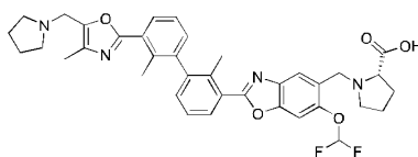
Compound 304
