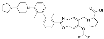
Compound 306
