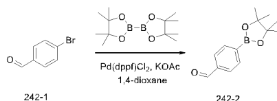
Compound 242
