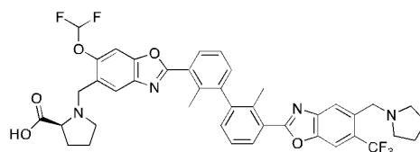
Compound 101
