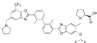
Compound 100
