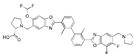
Compound 102
