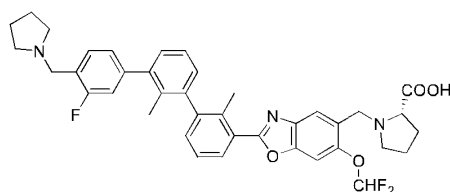
Compound 243
