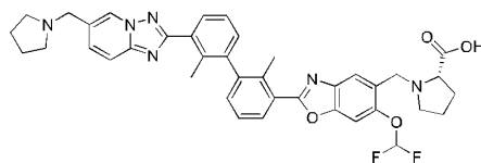
Compound 305
