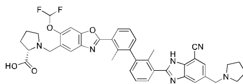
Compound 295
