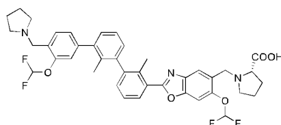
Compound 244
