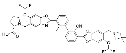
Compound 4
