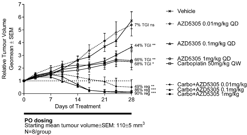
10 FIG. 8 Anti-tumour activity of AZD5305 in combination with carboplatin in HBCx-9 model
