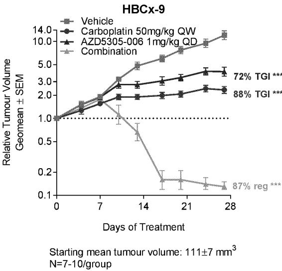
10 FIG. 2 Anti-tumour activity of AZD5305 in combination with carboplatin in HBCx-9 PDX model
