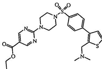
intermediate 82
