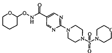
intermediate 36
