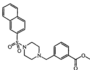
intermediate 11
