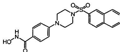
Compound 2
