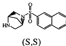
intermediate 43
