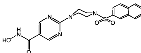
Compound 6
