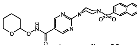
intermediate 33
