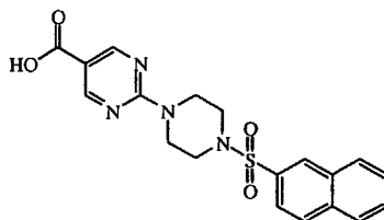
intermediate 32
