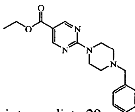
intermediate 29
