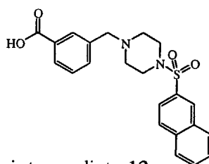
intermediate 12
