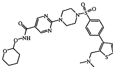
intermediate 84
