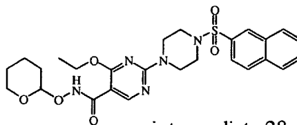
intermediate 28
