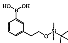
intermediate 92
