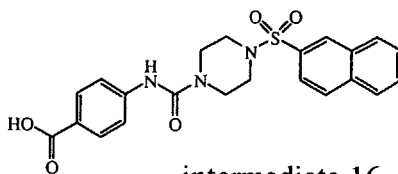
intermediate 16
