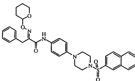
intermediate 20
