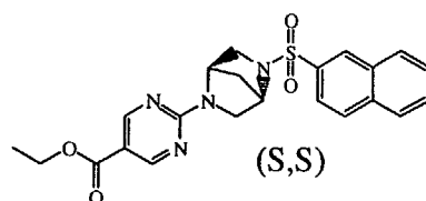
intermediate 44
