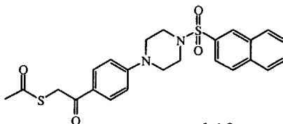
compound 10
