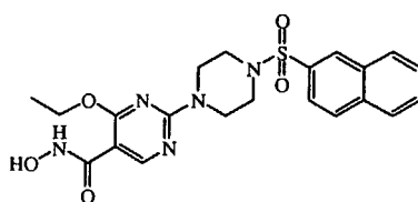
compound 12
