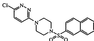
intermediate 41
