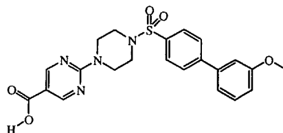
intermediate 39
