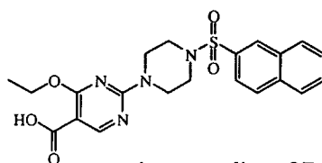
intermediate 27
