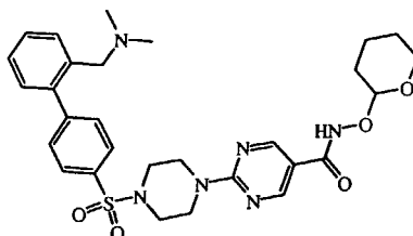
intermediate 91
