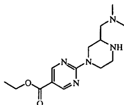
intermediate 76
