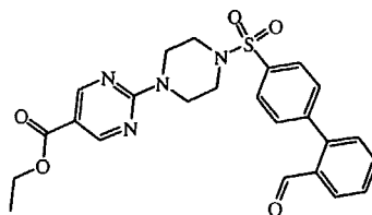
intermediate 88
