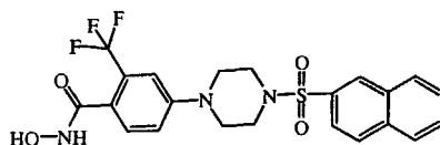
compound 11
