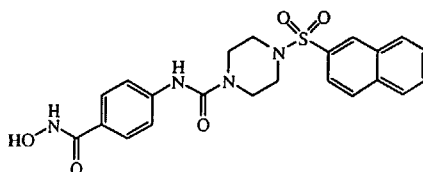
compound 8
