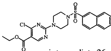
intermediate 26
