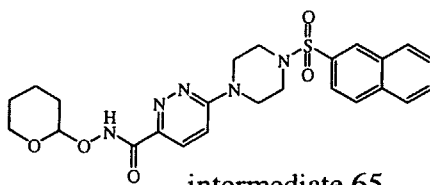
intermediate 65
