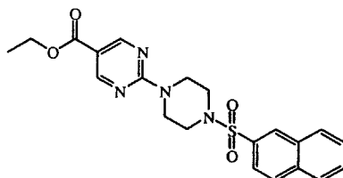
intermediate 31
