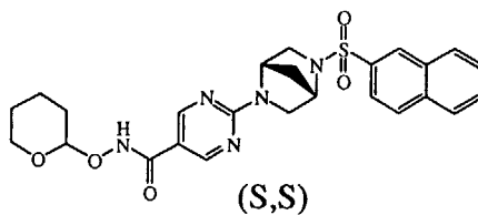
intermediate 46
