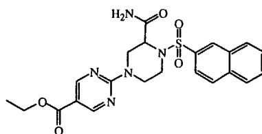
intermediate 58
