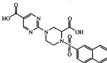
intermediate 74
