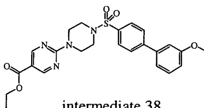
intermediate 38
