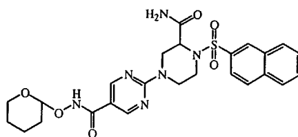
intermediate 60
