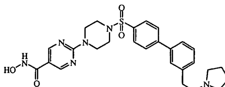
1.16 \text{C}_2\text{HF}_3\text{O}_2 compound 127
