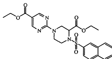
intermediate 73
