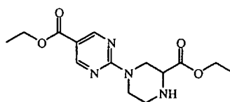
intermediate 72
