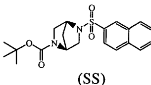
intermediate 42
