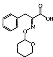
intermediate 19
