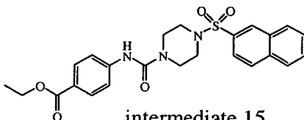
intermediate 15
