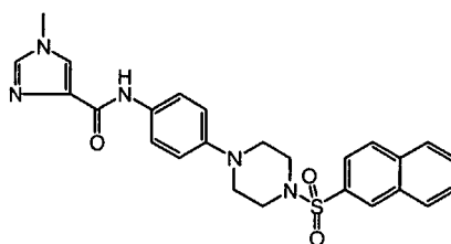
Compound 5
