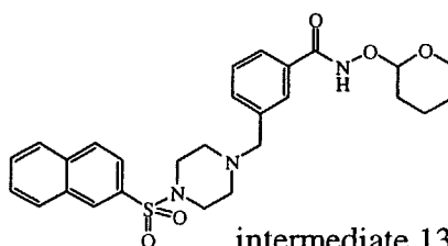
intermediate 13
