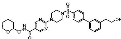
intermediate 102
