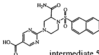
intermediate 59
