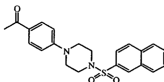
intermediate 21
