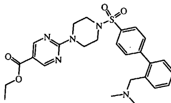
intermediate 89
