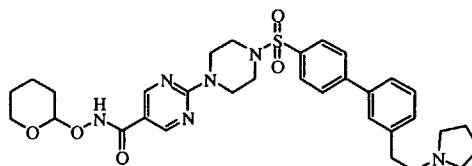
intermediate 97
