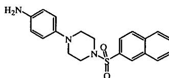
intermediate 18
