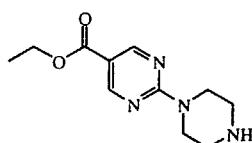
intermediate 30
