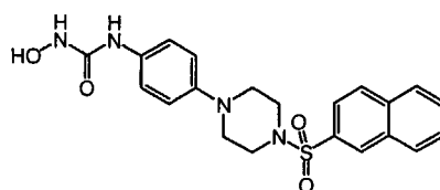
Compound 4
