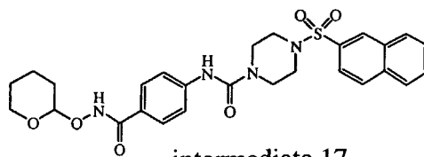
intermediate 17
