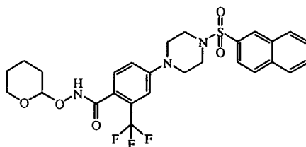
intermediate 25
