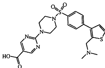
intermediate 83
