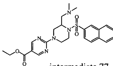
intermediate 77
