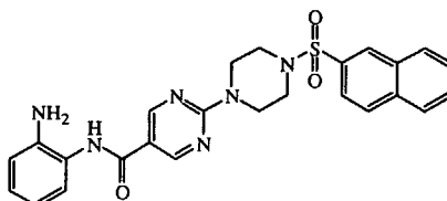
compound 13
