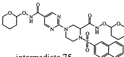
intermediate 75
