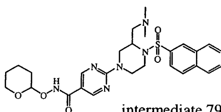
intermediate 79
