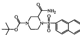
intermediate 56
