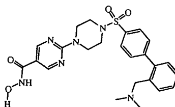
\cdot\text{C}_2\text{HF}_3\text{O}_2 compound 126
