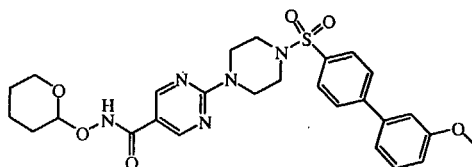
intermediate 40
