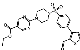
intermediate 81
