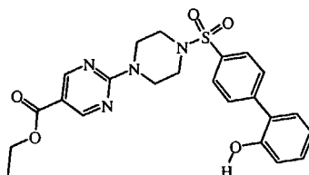
intermediate 85
