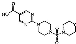
intermediate 35
