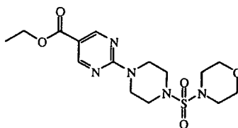
intermediate 34
