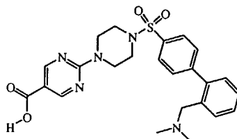
intermediate 90
