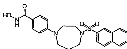
Compound 1
