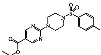
intermediate 37
