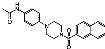
Compound 3
