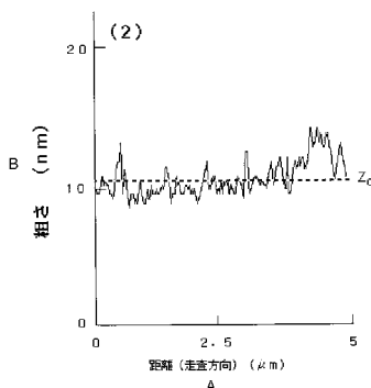
A...DISTANCE (SCANNING DIRECTION) (μm) B...ROUGHNESS (nm) C...SCALE OF HEIGHT (ROUGHNESS) D...THE PART SCANNED
