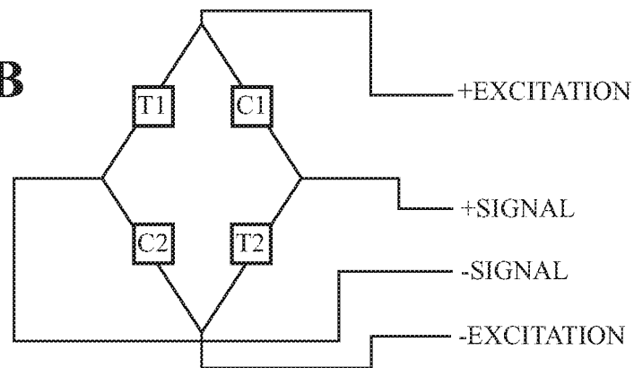
Full Bridge Schematic 2
