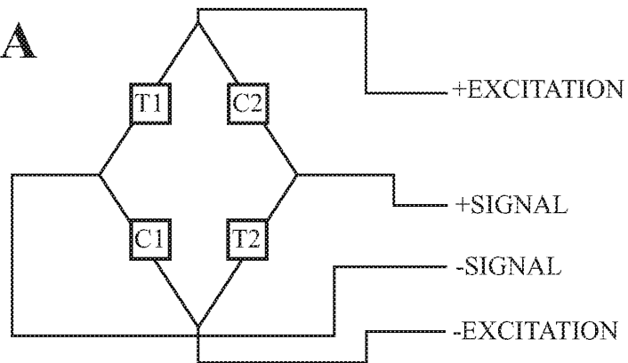
Full Bridge Schematic 1
