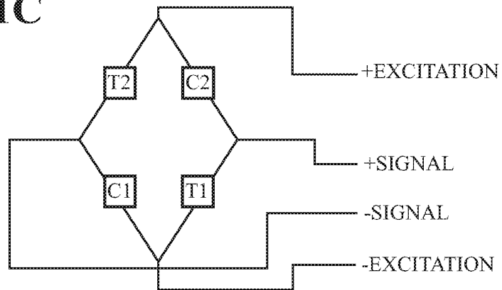
Full Bridge Schematic 3
