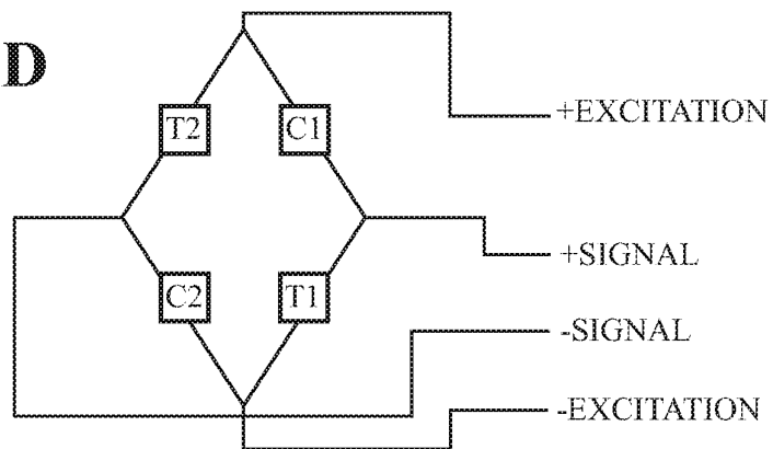
Full Bridge Schematic 4
