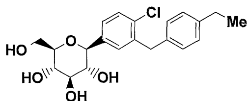
Compound 1 (a compound of formula I).
