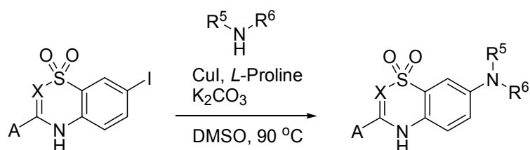
Scheme 28
