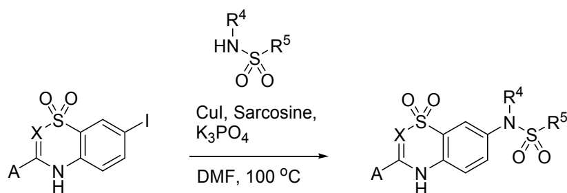
Scheme 24
