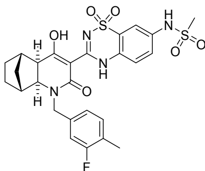
a) (1 S ,2 R ,3 S ,4 R )-3-(3-Fluoro-4-methyl-benzylamino)-bicyclo[2.2.1]heptane-2-carboxylic acid ethyl ester
