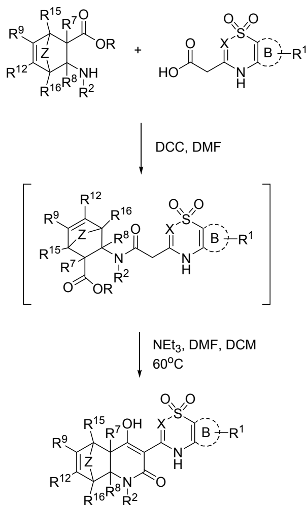
Scheme 2
