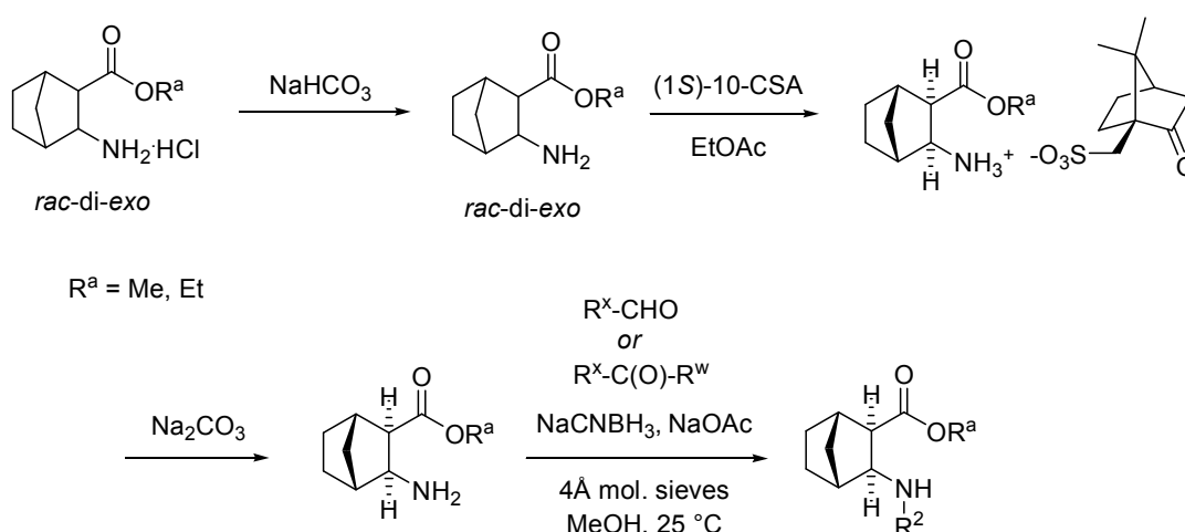
Scheme 7
