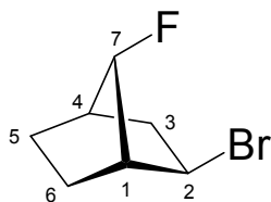
2-exo-bromo-7-syn-fluoro-bicyclo[2.2.1]heptane
