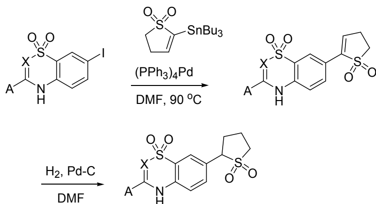
Scheme 27
