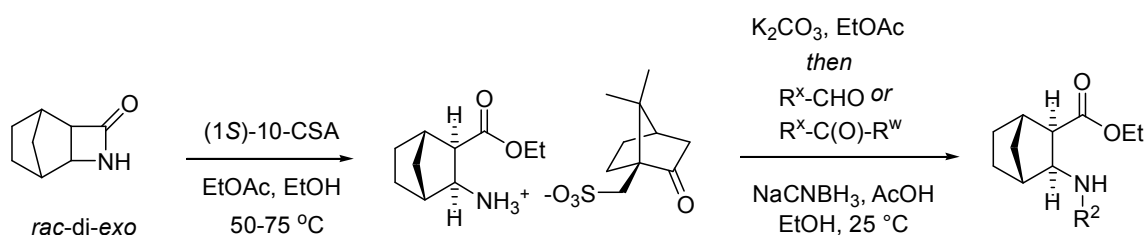
Scheme 8
