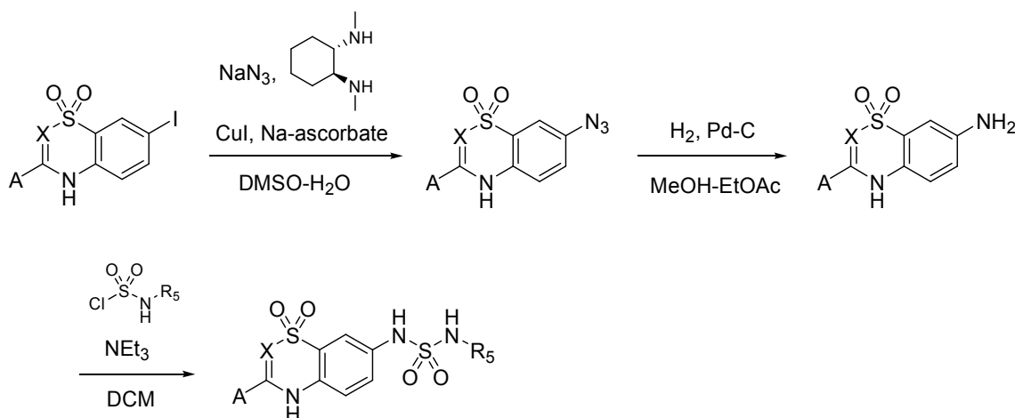
Scheme 25
