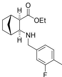
a) (1 S ,2 R ,3 S ,4 R )-3-(3-Fluoro-4-methyl-benzylamino)-bicyclo[2.2.1]heptane-2-carboxylic acid ethyl ester
