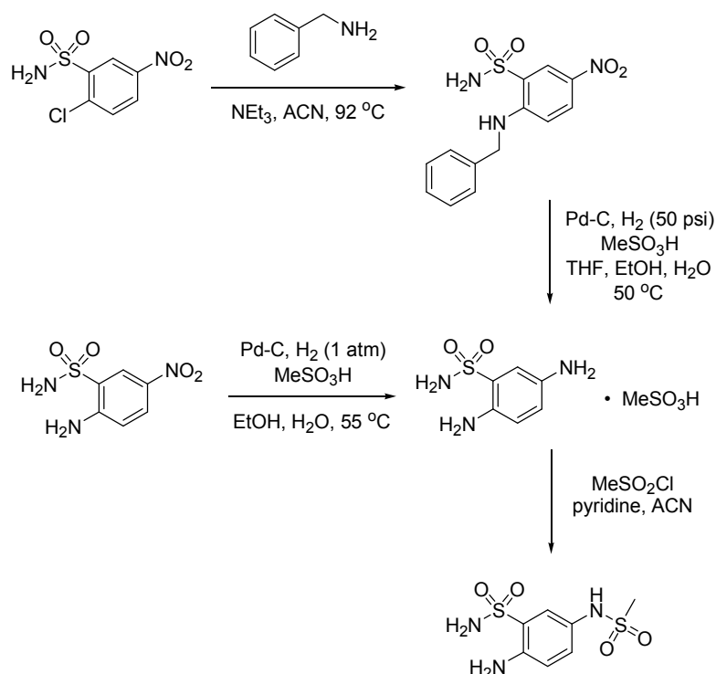
Scheme 16
