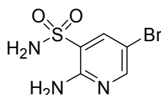
a) 2-Amino-5-bromo-pyridine-3-sulfonic acid amide
