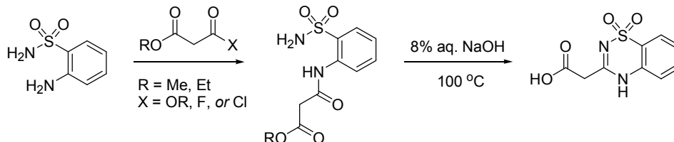
Scheme 18
