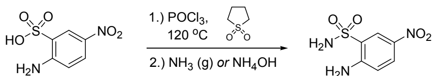
Scheme 15
