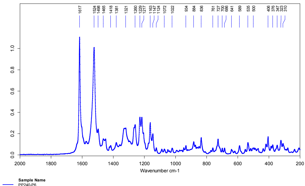
Graph 2. FT-Raman Spectrum.
