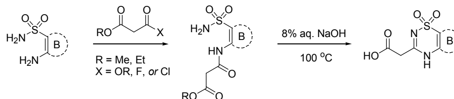
Scheme 23
