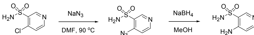
Scheme 22
