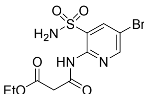
b) N -(5-Bromo-3-sulfamoyl-pyridin-2-yl)-malonamic acid ethyl ester
