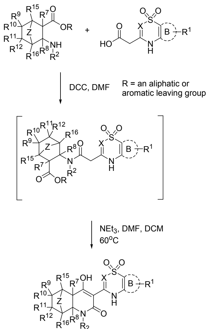
Scheme 1
