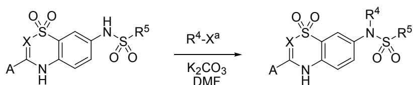
Scheme 26
