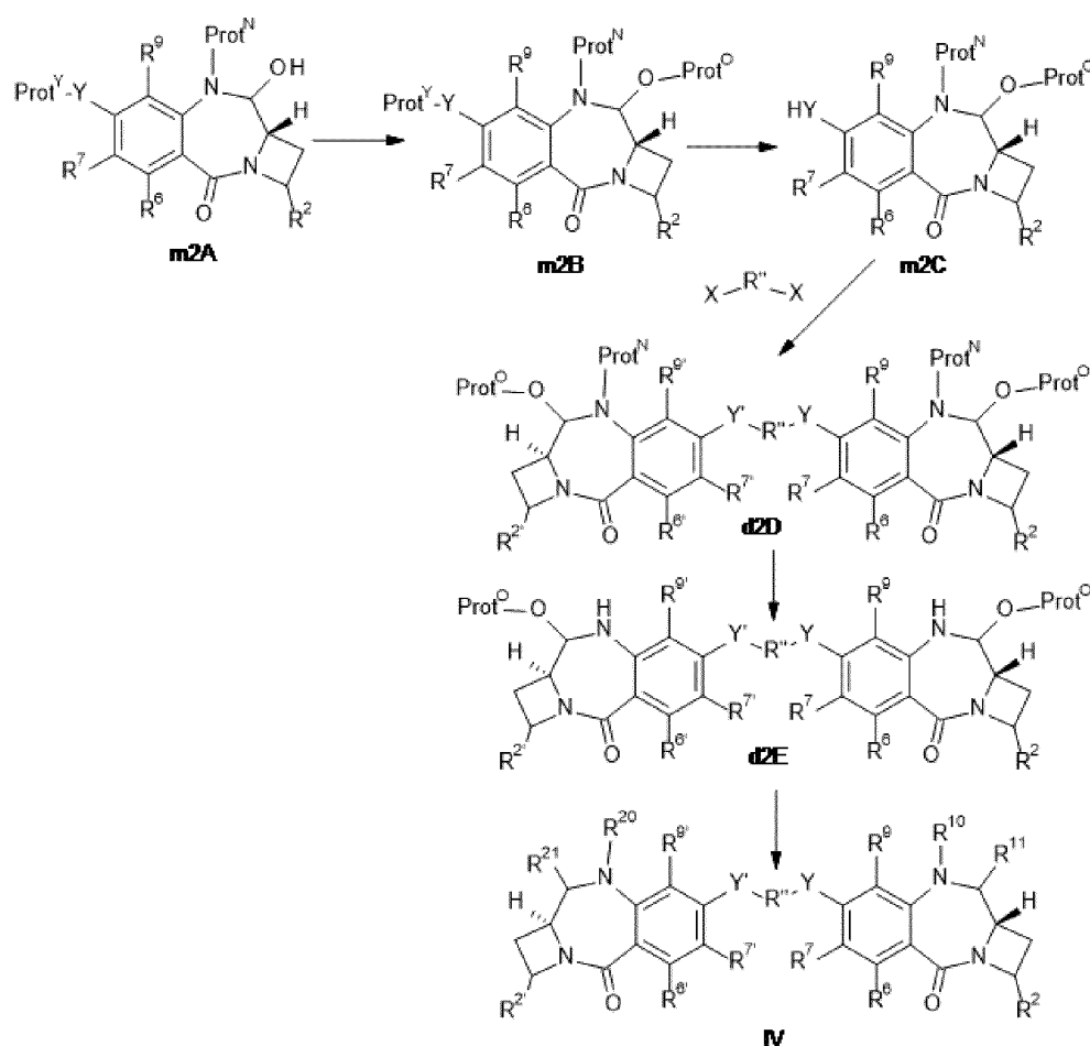
Scheme 2
