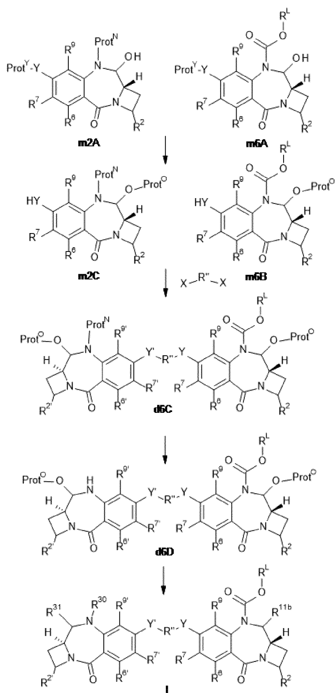
Scheme 6
