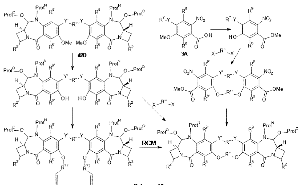
Scheme 10
