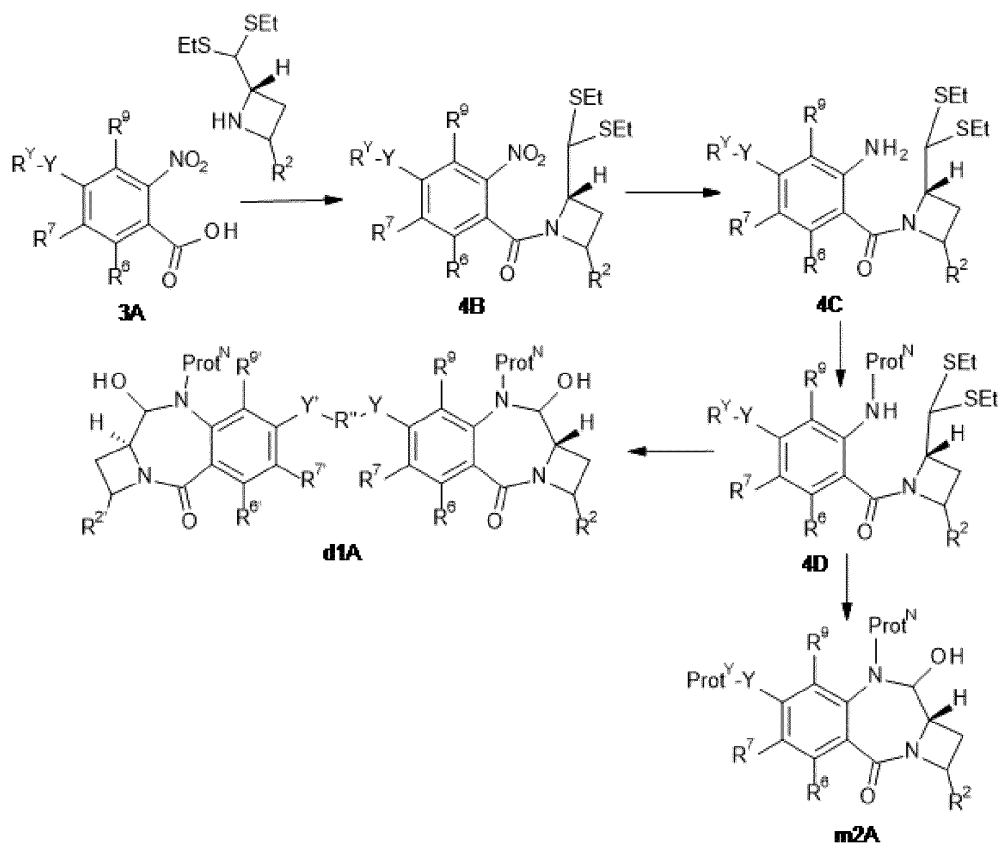
Scheme 4
