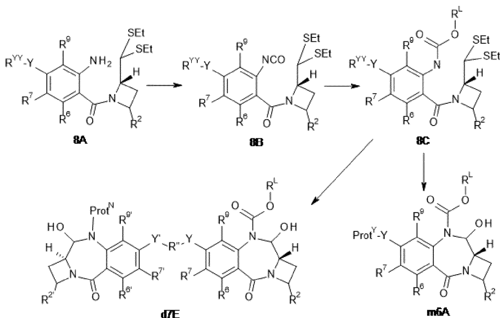
Scheme 8
