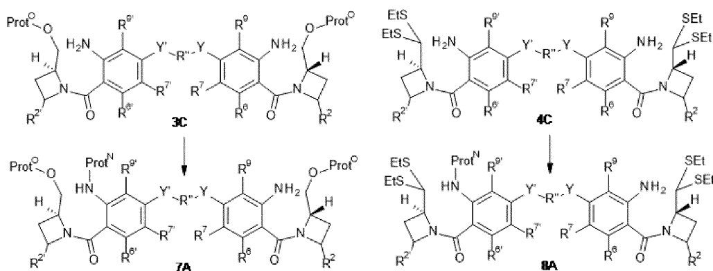
Scheme 9
