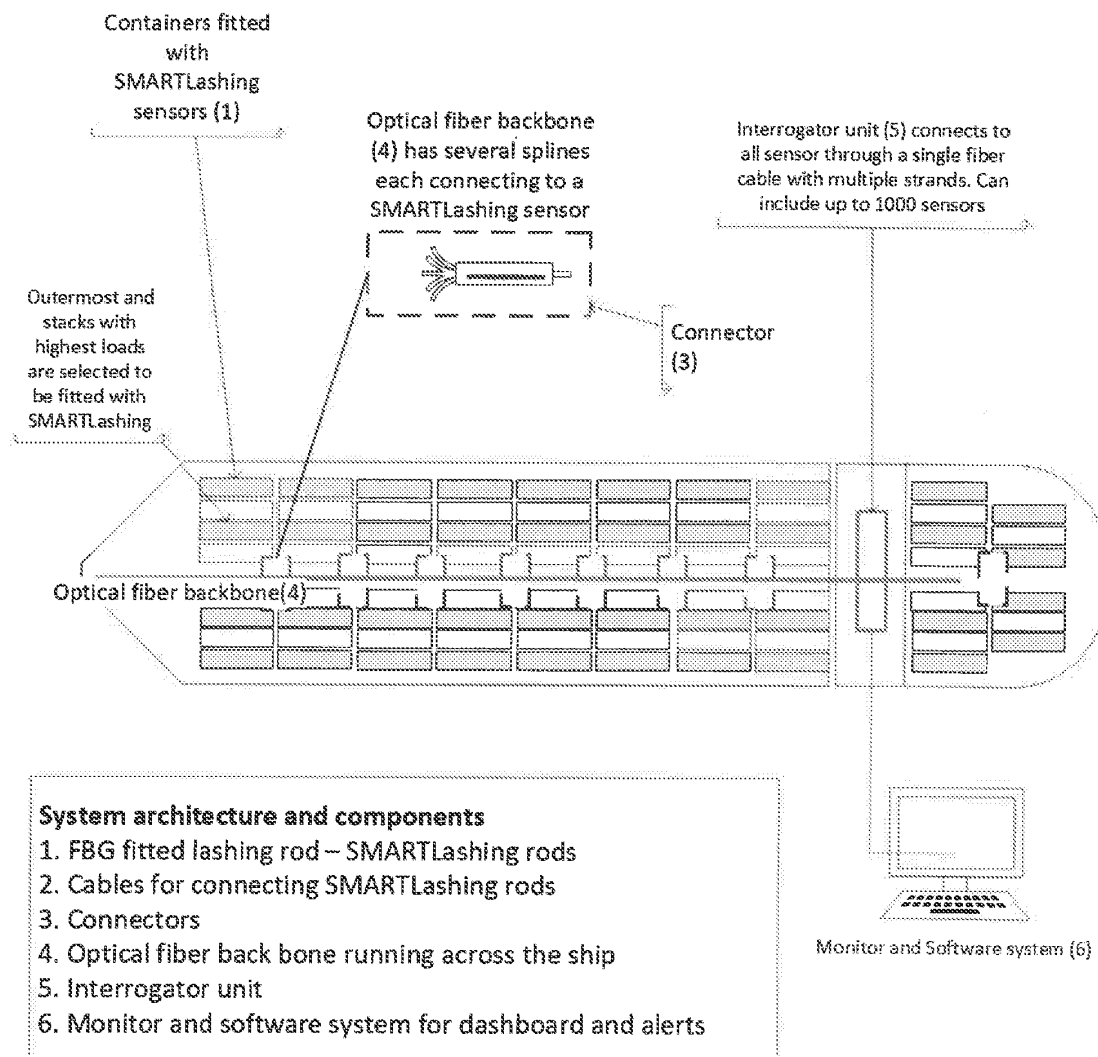
SMARTLashing system architecture diagram
