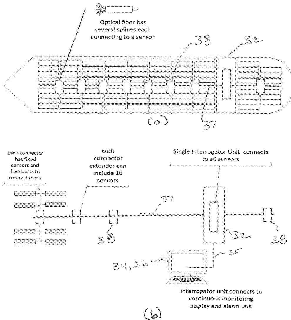
Schematic design and cable layout for lashing monitoring system
