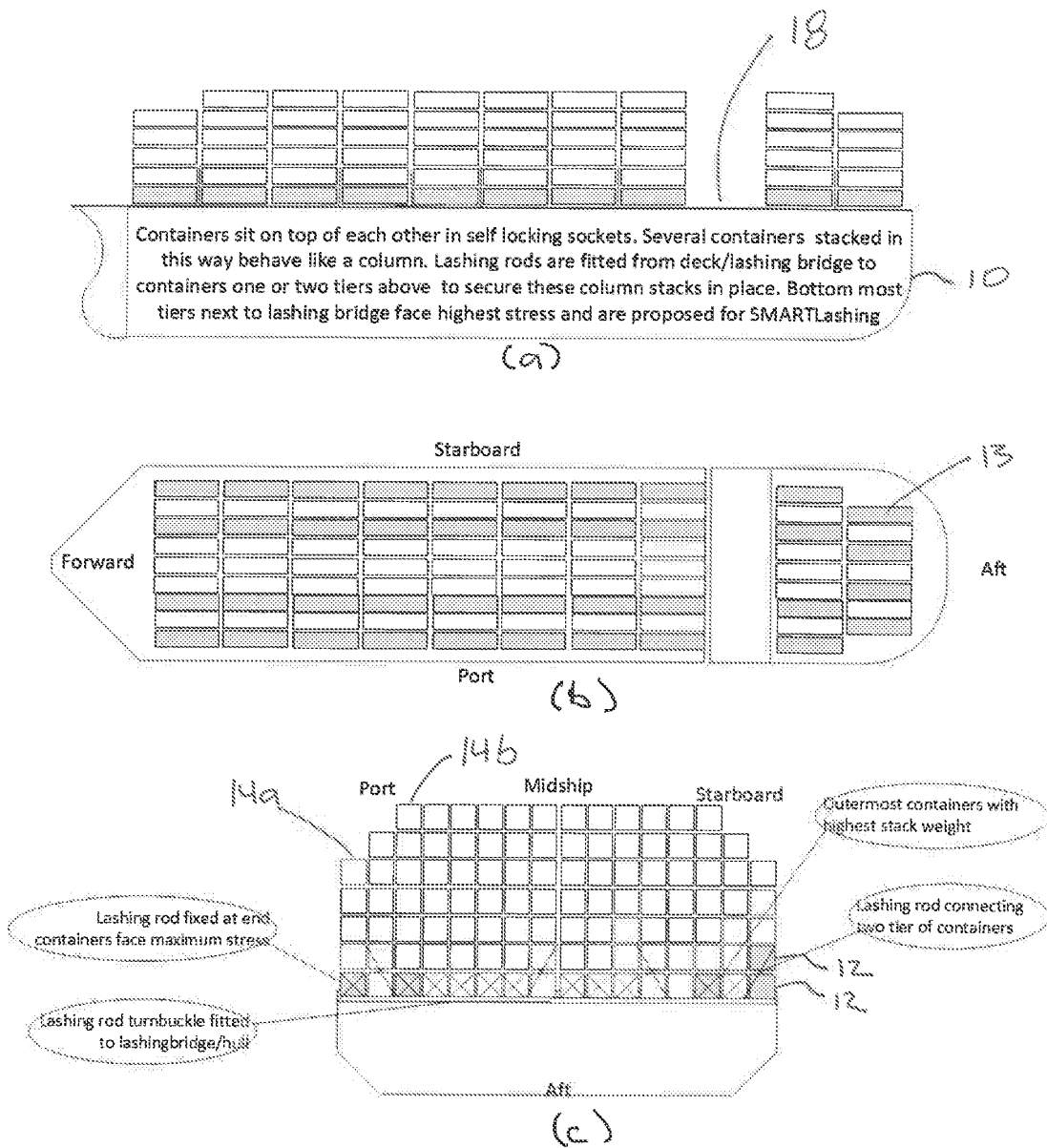
Schematic layout for containers fitted with SMARTLashing system
