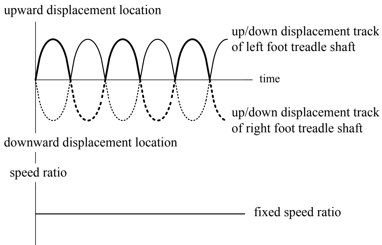
FIG. 1 (Prior Art)
