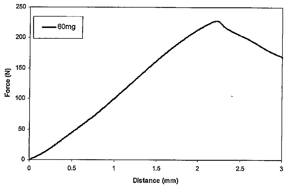
Example 20 Indentation Test of Example 16.1 tablet
