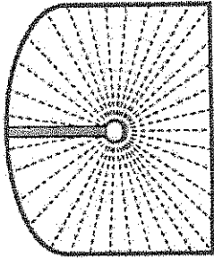
FIGURE 2C: +270° COVERAGE
