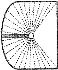
FIGURE 2A: +90° COVERAGE
