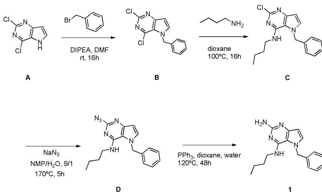
Scheme 1. Overall reaction scheme
