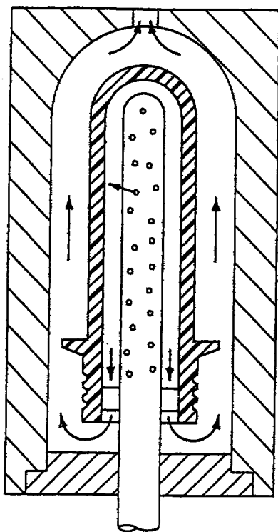
FIG. 21 (PRIOR ART)
