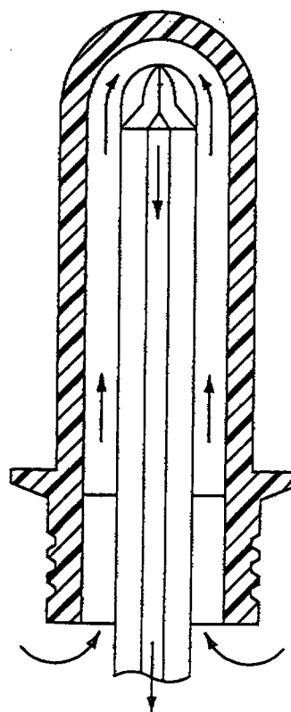
FIG. 22 (PRIOR ART)
